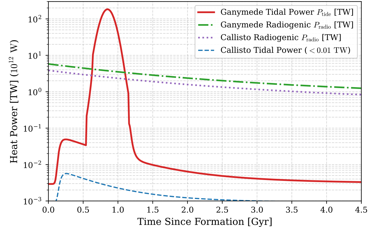
(c) Thermal Power Source Breakdown
