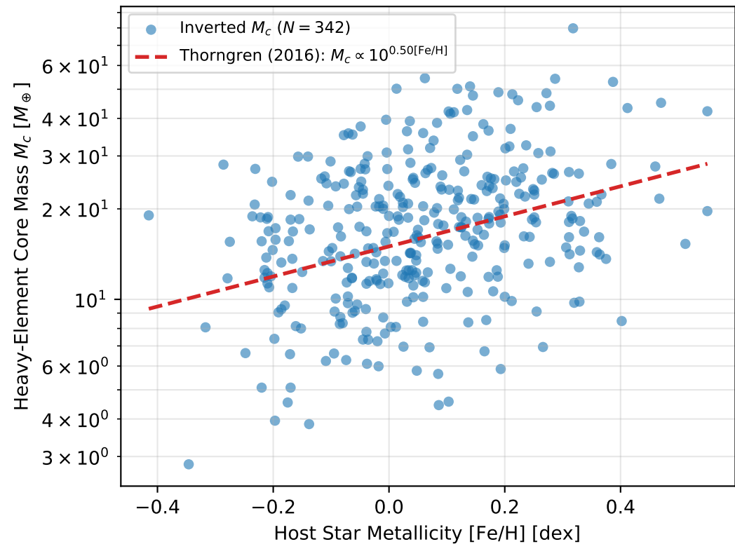
(a) Heavy-Element Mass M_c [ M_\oplus ]
