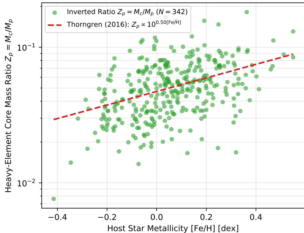
(b) Heavy-Element Ratio Z_p = M_c/M_p
