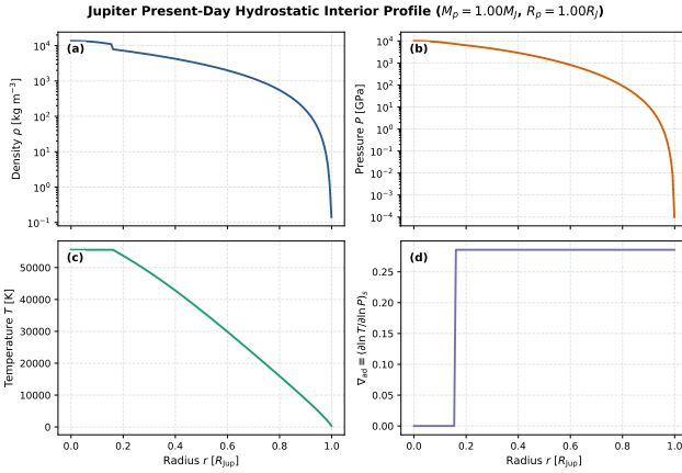
Figure 2: Scenario 1: 1D interior hydrostatic profile ( \rho, P, T, \nabla_{\text{ad}} ) of present-day Jupiter at 4.56 \text{ Gyr} , demonstrating smooth un-truncated radial coverage from core ( r/R_p = 0.00 ) to atmosphere (1.00).
