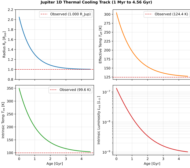
Figure 1: Scenario 1: 4-Panel diagnostic thermal cooling track for Jupiter ( M_p = 1.00 M_{\text{Jup}} , M_c = 12.0 M_{\oplus} , a = 5.204 \text{ AU} ) from t = 1 \text{ Myr} to 4.56 \text{ Gyr} .
