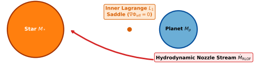
Figure 19: Roche lobe equipotential surfaces and hydrodynamic nozzle escape through L_1 .
