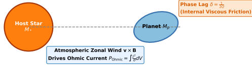
Figure 18: Quadrupolar tidal flexure and lagging tidal bulge geometry.
