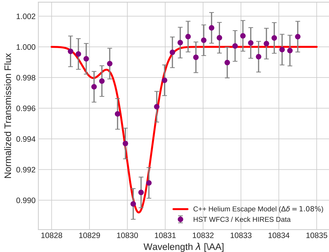
HAT-P-11b High-Res He I 10830\AA\ Transmission
