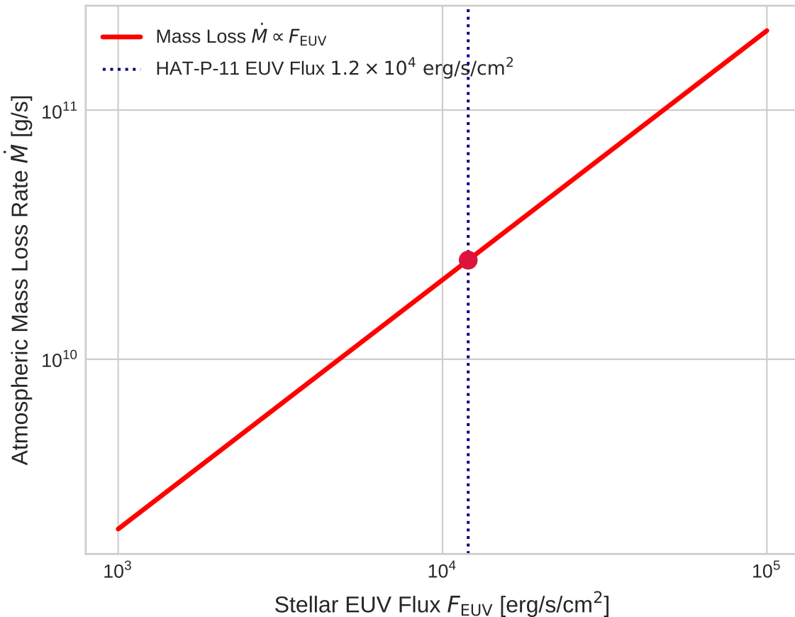
Model Choice: Mass Loss vs EUV Flux
