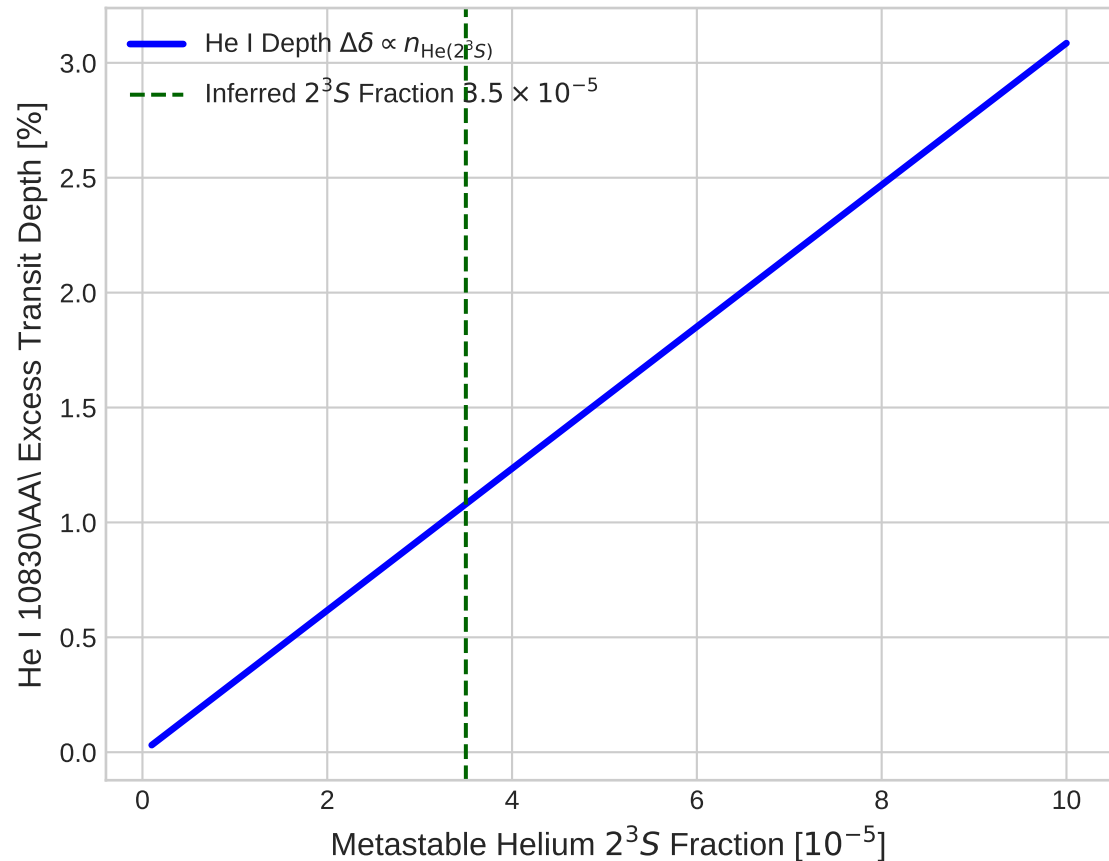
Model Choice: Triplet Population Sensitivity
