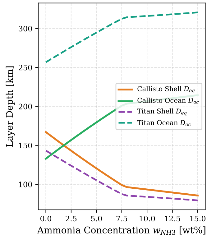
(c) Ammonia Antifreeze Effect
