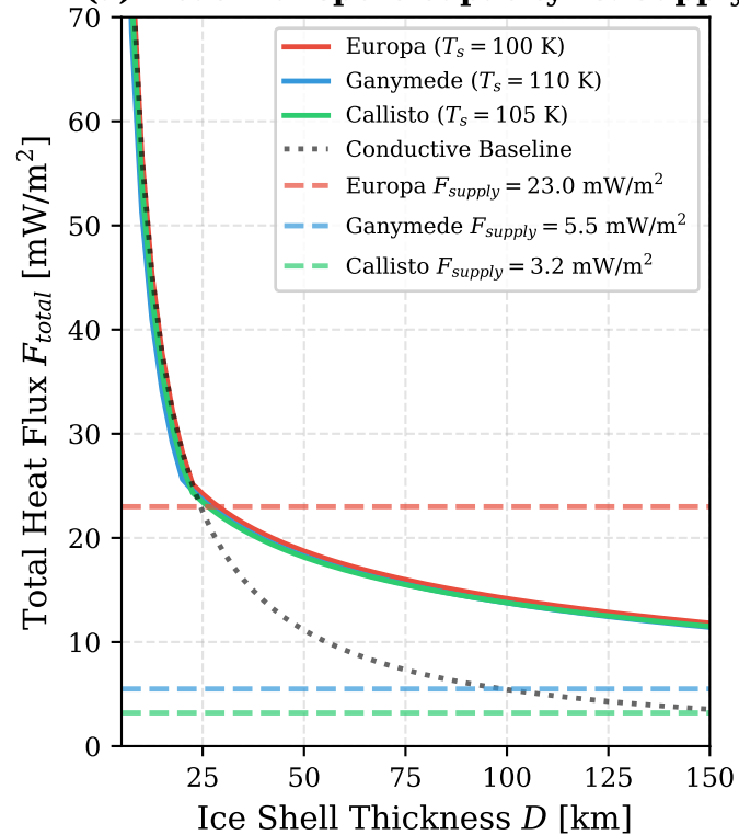
(a) Heat Transport Capacity vs. Supply
