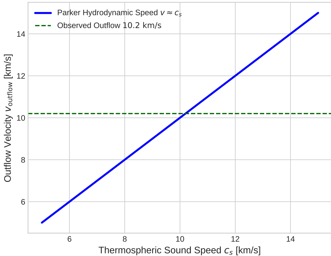
Model Choice: Wind Velocity Profile
