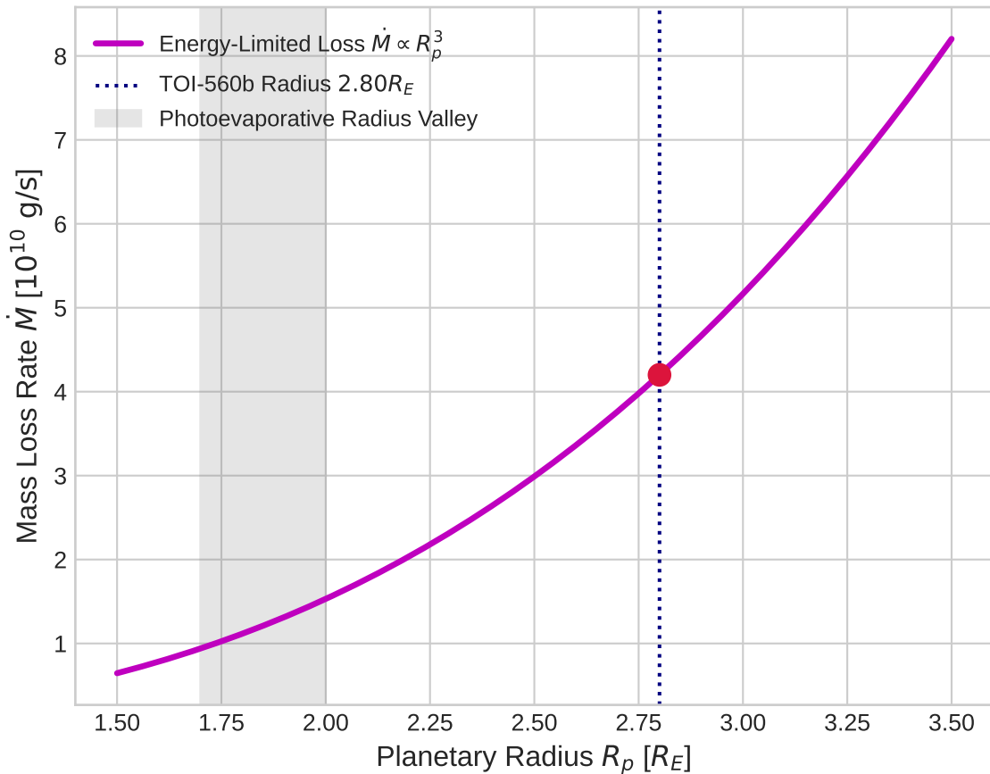
Model Choice: Mass Loss & Radius Evolution
