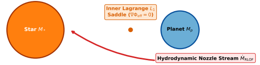
Derivation A9: Roche Lobe Overflow (RLOF) & Mass Loss
