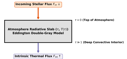
Figure 17: Two-stream double-gray radiative boundary geometry under stellar irradiation.
