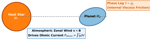
Derivation A6: Tidal Bulge Deformation & Ohmic Dissipation
