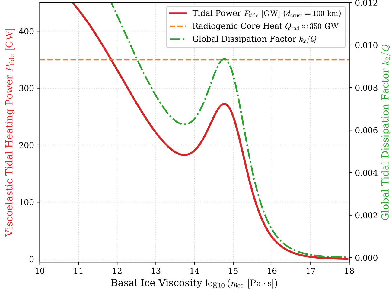
(b) Interior Tidal Heat Production & Thermal Balance
