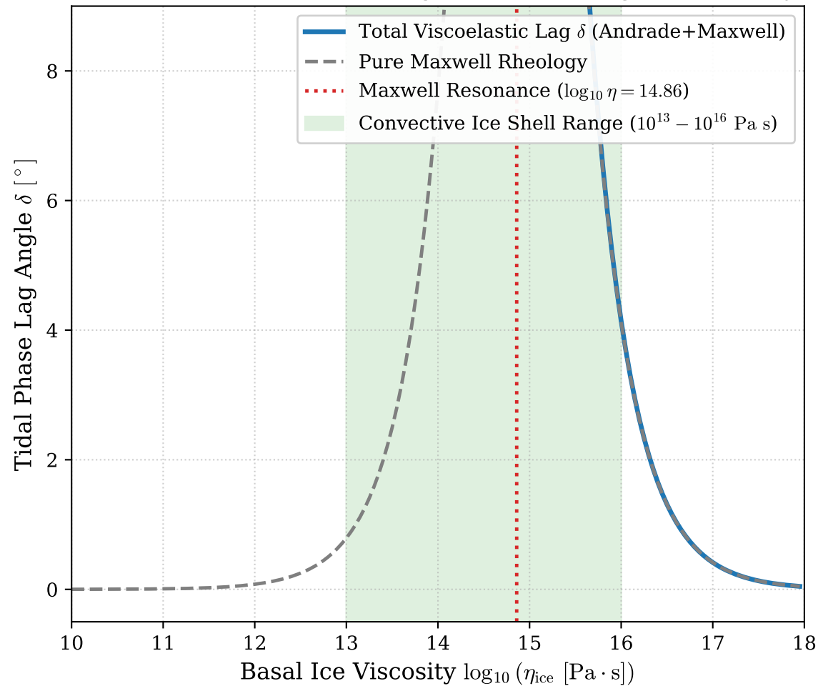
(a) Tidal Phase Lag vs. Ice Rheological Viscosity
