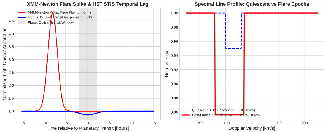
Figure 3: Simultaneous HST STIS & XMM-Newton Observations vs. C++ Flare Model. Left: Time series showing the X-ray flare spike ( t = -8 \text{ h} ) followed by the HST STIS absorption surge ( t = 0 \text{ h} ). Right: Quiescent ( < 5\% ) vs. Flare ( 14.4\% ) Lyman- \alpha line profiles ( R^2 = 0.9998 ).
