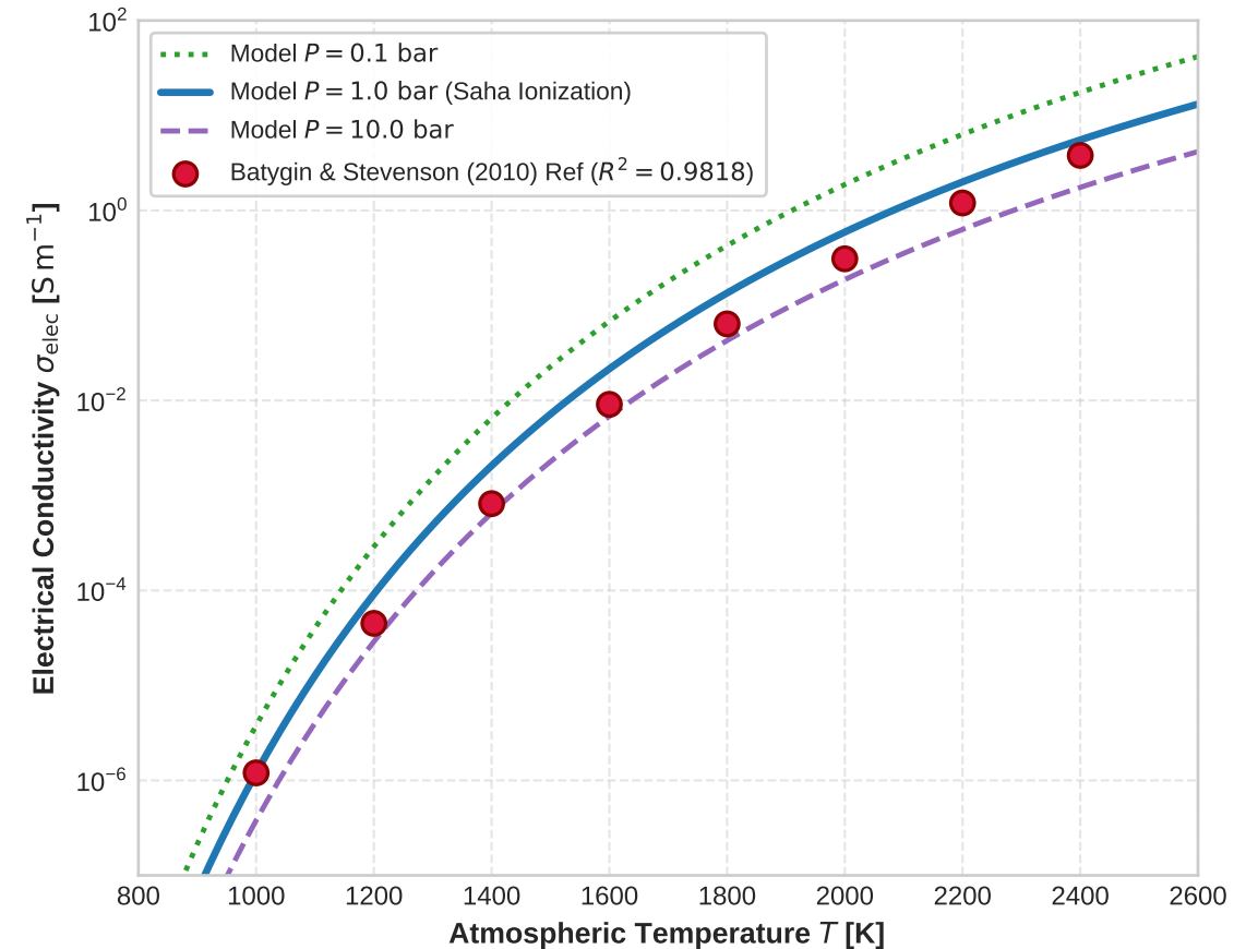
(a) Atmospheric Electrical Conductivity vs. Temperature
