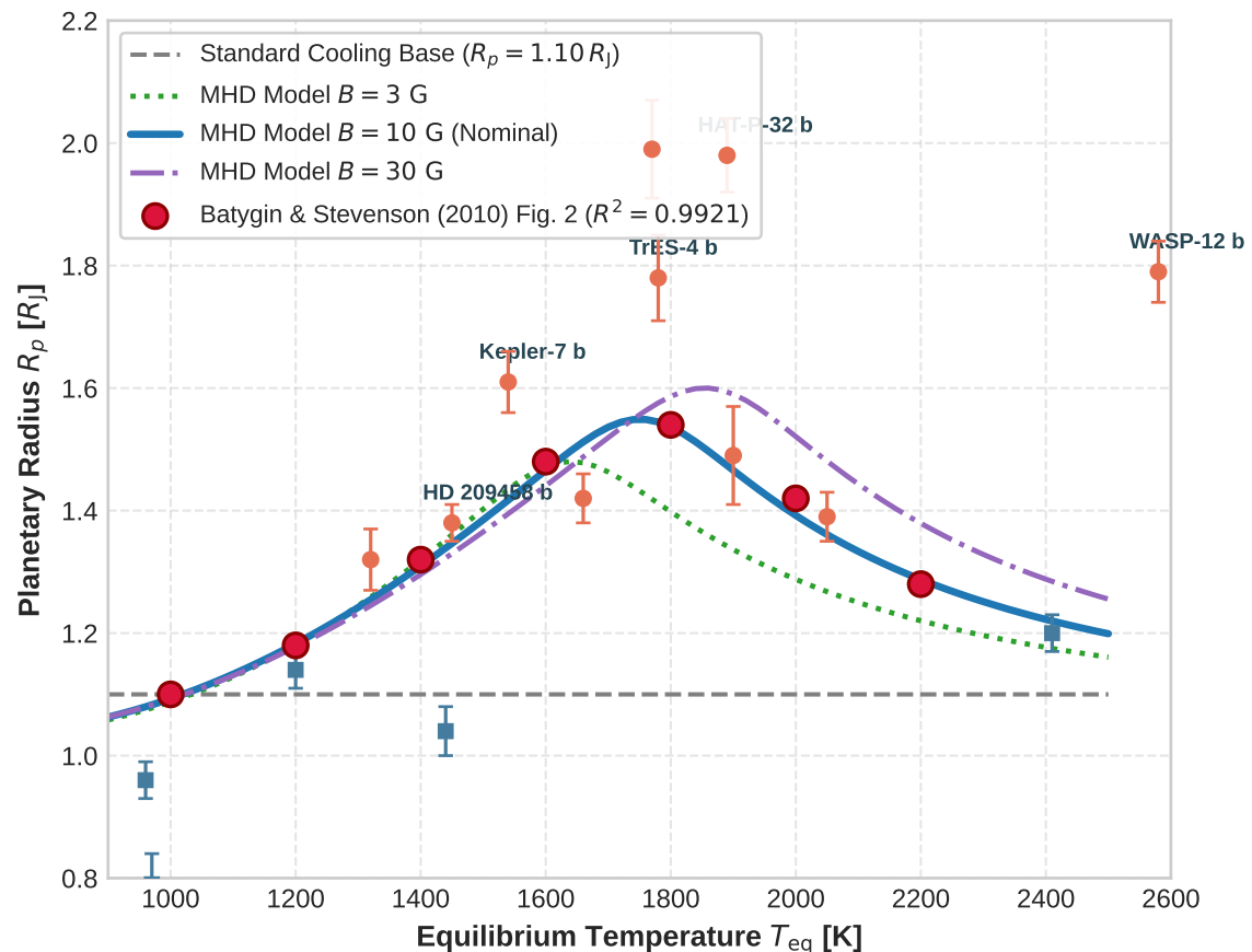
(b) Ohmic Radius Inflation Peak vs. Equilibrium Temperature
