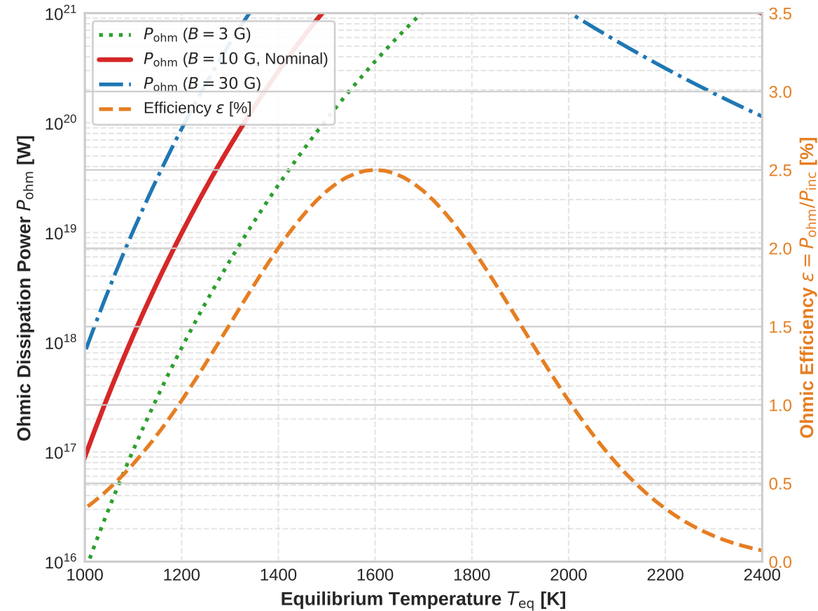
(a) Integrated Ohmic Heating Power & Conversion Efficiency
