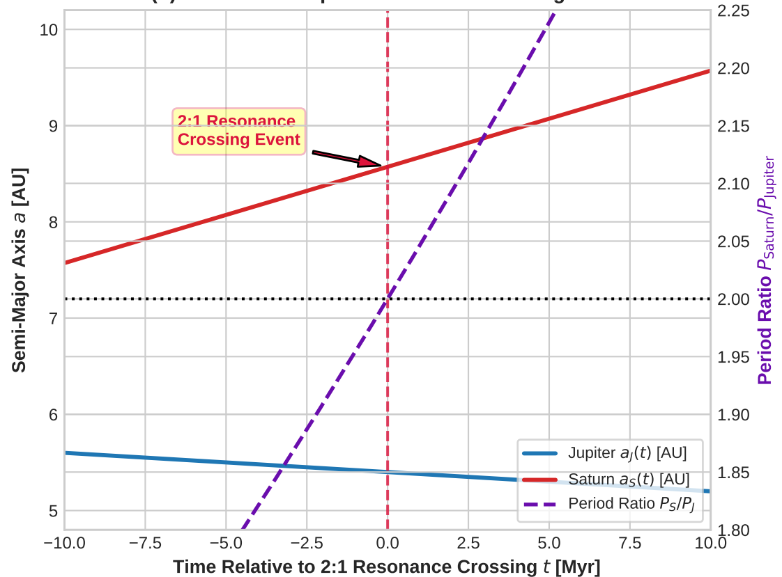
(b) Nice Model Jupiter-Saturn 2:1 Crossing Track
