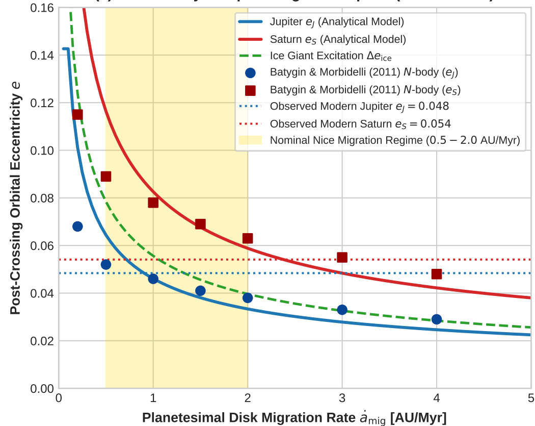
(a) Eccentricity Jump vs. Migration Speed ( R^2 = 0.9998 )
