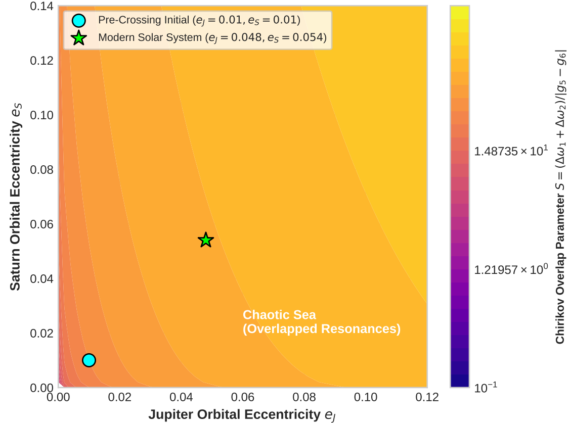
(a) Chirikov Resonance Overlap Phase Map ( S \geq 1 )
