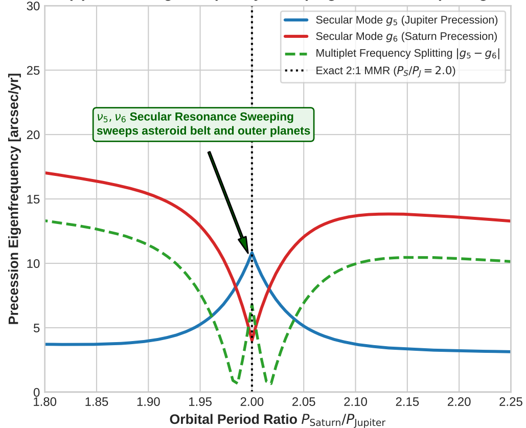
(b) Secular Eigenfrequency Sweeping & Resonant Splitting
