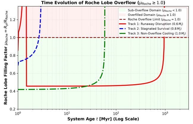
Figure 2: Roche Lobe Radius Contraction and Filling Factor. Time evolution of filling factor \mu_{\text{Roche}}(t) = R_p/R_{\text{Roche}} . Overflowing ( \mu_{\text{Roche}} \geq 1.0 , red shaded region) initiates hydrodynamic mass loss, while sub-overflow ( \mu_{\text{Roche}} < 1.0 , green shaded region) represents stable cooling.
