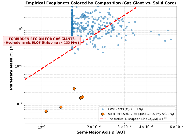
Figure 4: Empirical Gas Giant Truncation Boundary. Observed transiting exoplanet population from hot_jupiter.db overlaid with the theoretical RLOF disruption boundary (red dashed curve), color-coded by planet composition (blue circles: Gas Giants M_p \geq 0.1 M_{Jup} ; orange diamonds: Solid Terrestrial Cores M_p < 0.1 M_{Jup} ).
