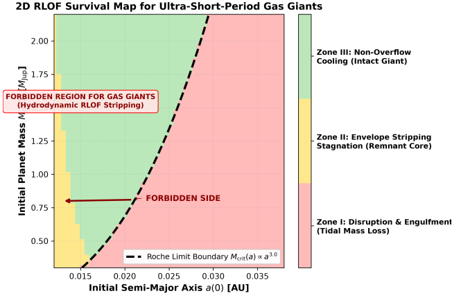
Figure 3: Survival Phase Space Diagram & Trajectory Flow. 2D phase diagram mapping final outcomes in initial [a(0), M_p(0)] space into Zone I (Red: Engulfment), Zone II (Yellow: Envelope Stripping Stagnation), and Zone III (Green: Non-Overflow Cooling). The black dashed line denotes the analytical Roche limit M_{crit}(a) \propto a^{3.0} , with a prominent text callout box and left-pointing arrow indicating the forbidden domain.
