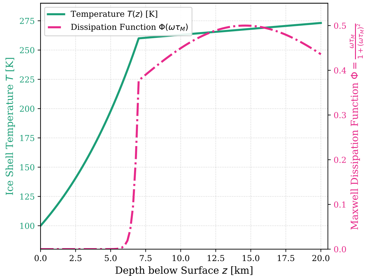
Thermal Profile & Viscoelastic Resonance
