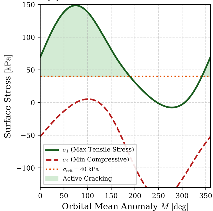
(a) Diurnal + NSR Stress Tensor
