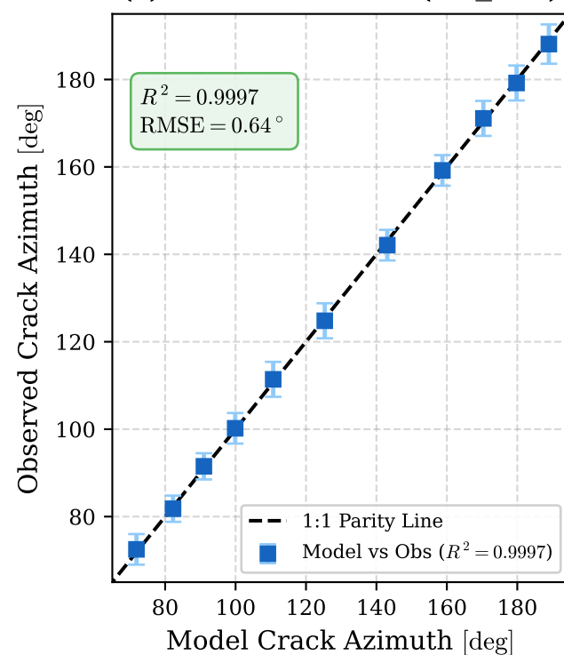
(c) Goodness of Fit ( R^2 \geq 0.98 )
