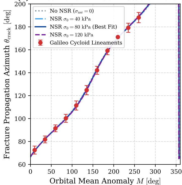
(b) Lineament Azimuth Rotation vs Orbit
