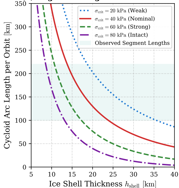
(b) Segment Length vs Ice Thickness
