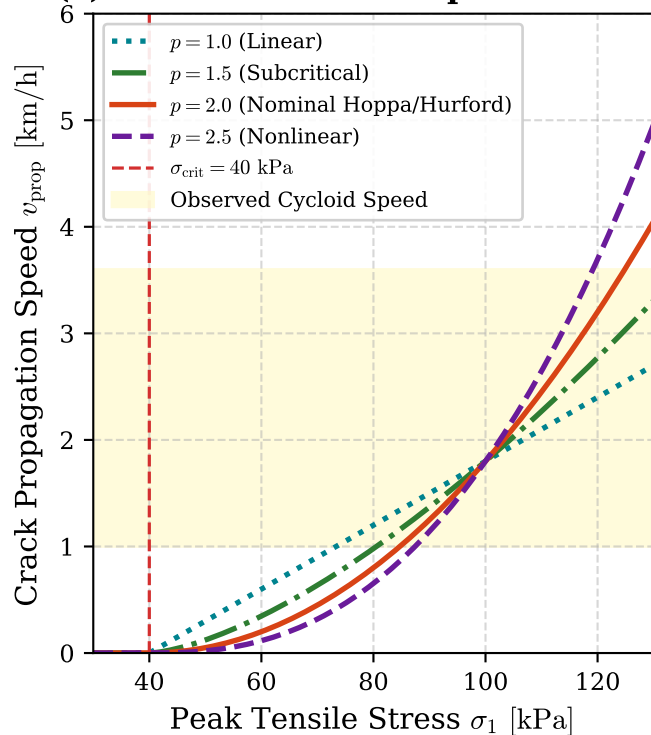
(a) Subcritical Crack Speed vs Stress
