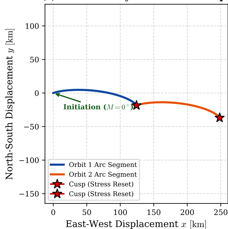
(c) Simulated Cycloid Path & Cusps
