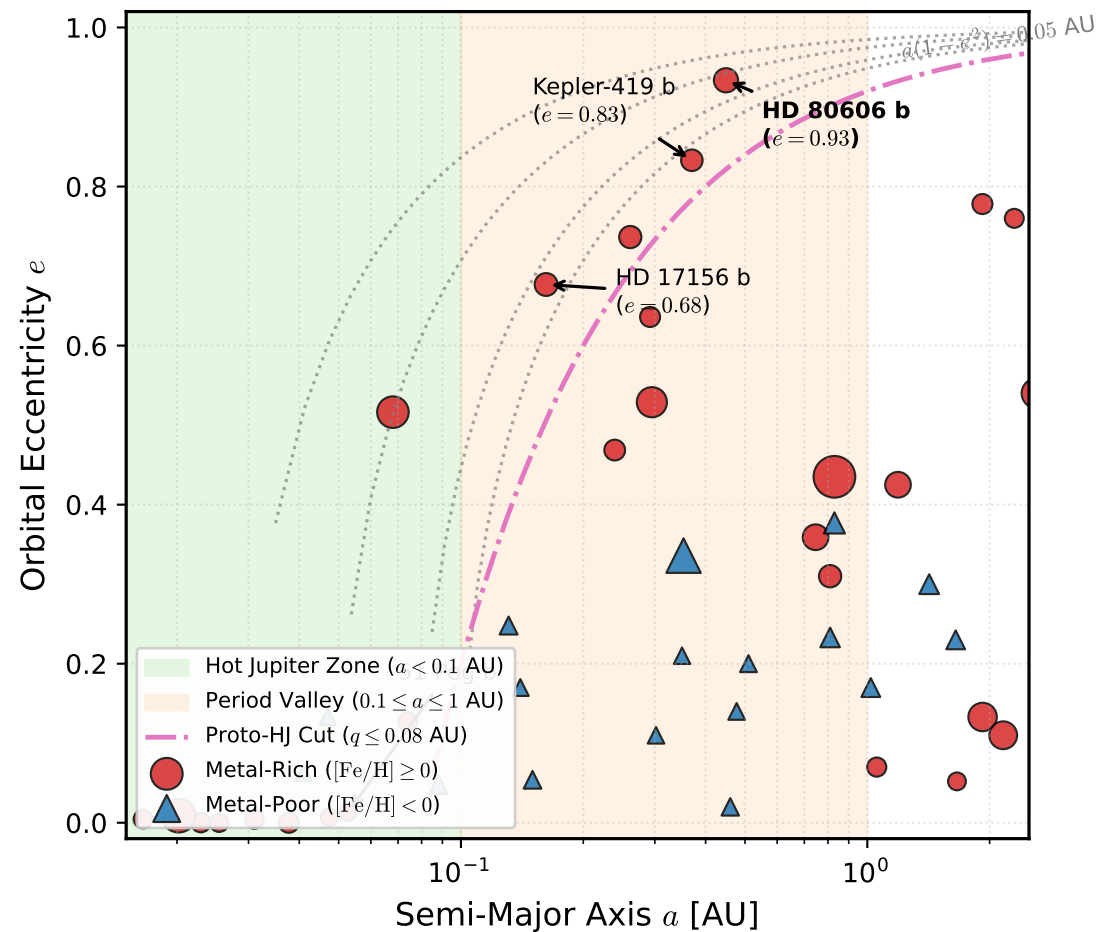
(b) e vs a Exoplanet Demographics
