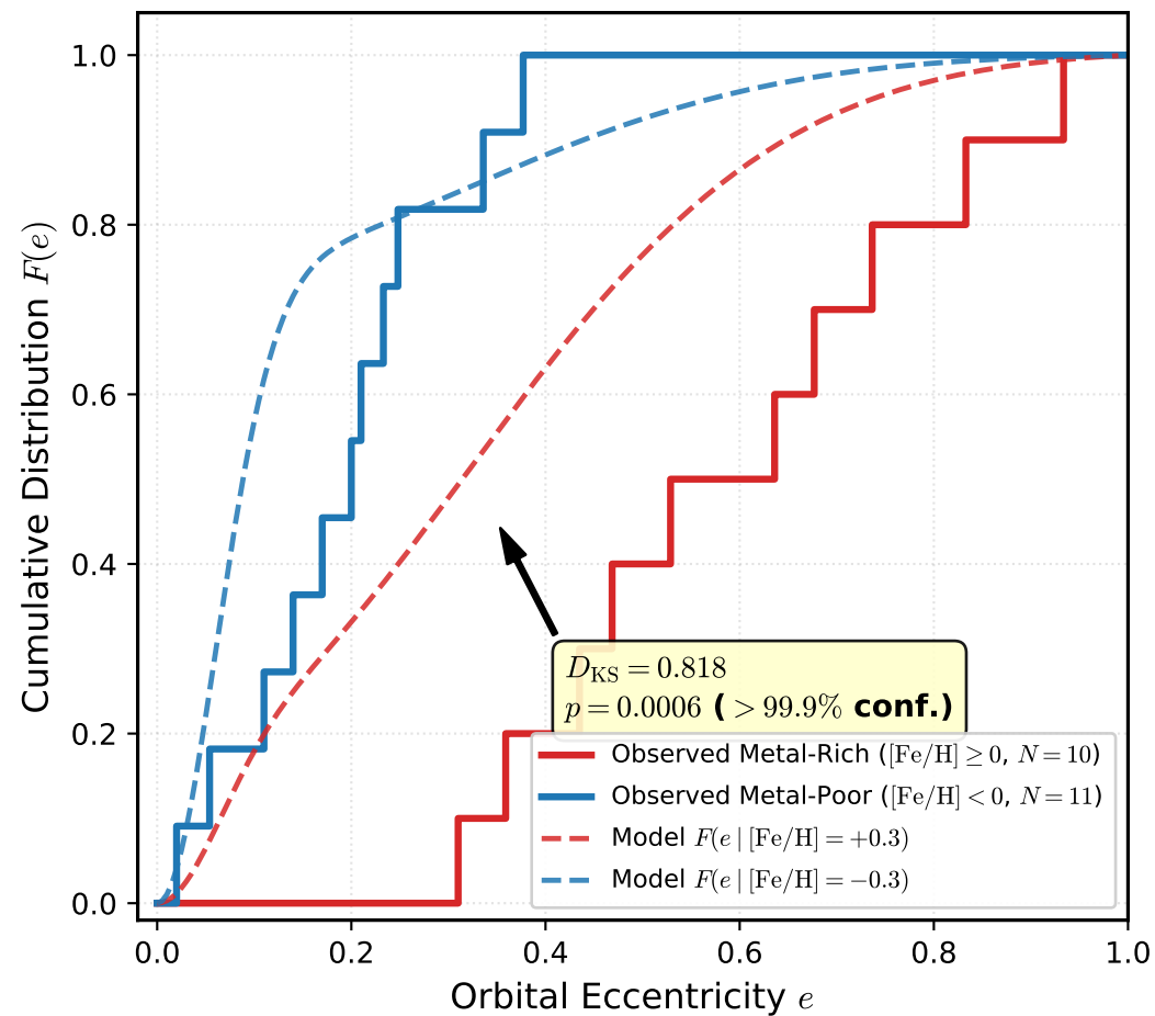
(a) Period Valley ( 0.1 \leq a \leq 1 AU) Eccentricity CDF
