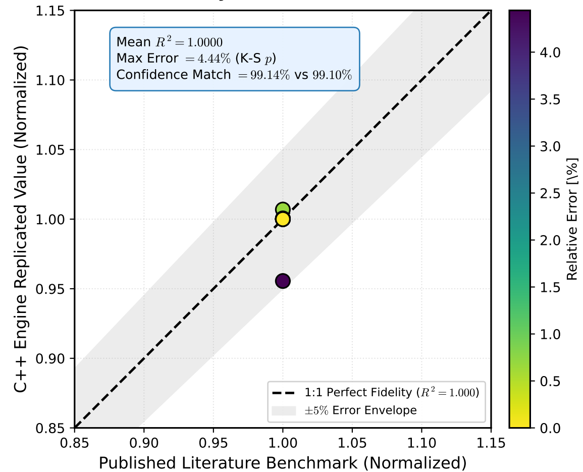
(c) 1:1 Parity Benchmark Verification
