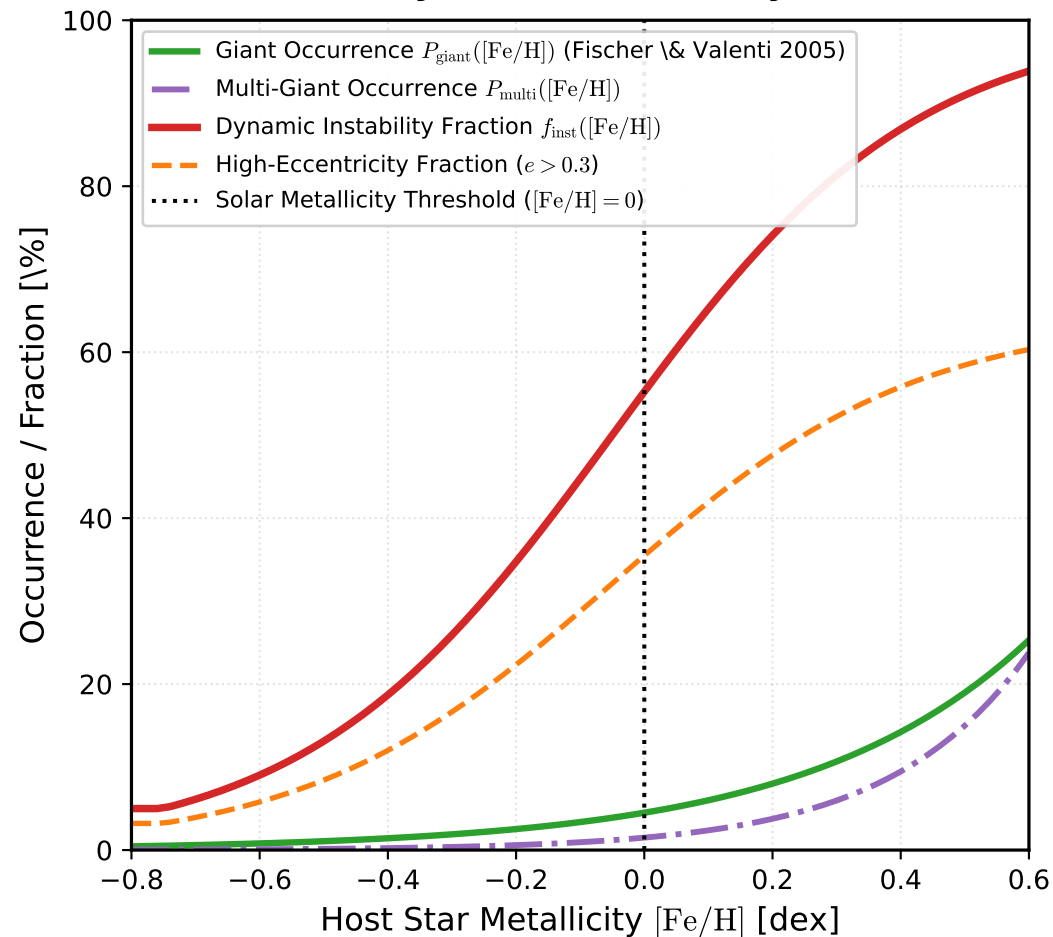
(a) Metallicity-Driven Instability Transition
