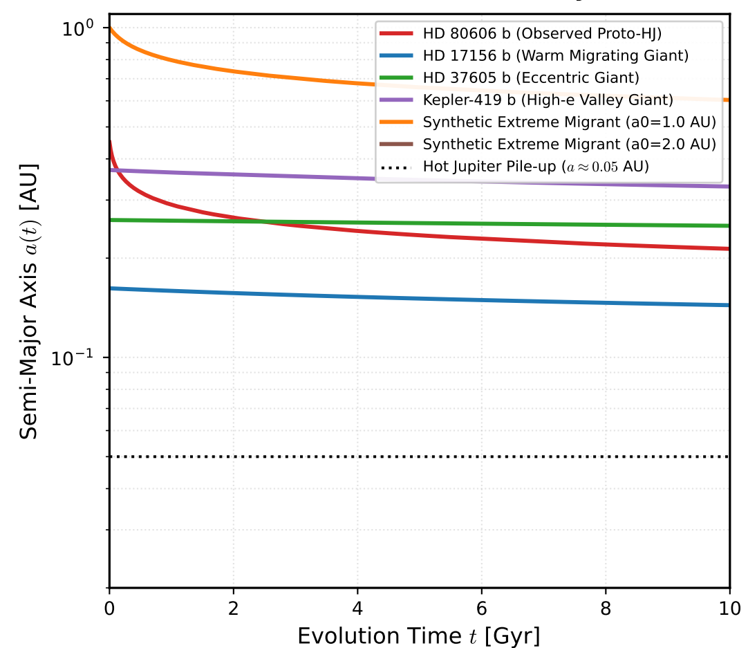
(c) Tidal Circularization & Decay Tracks
