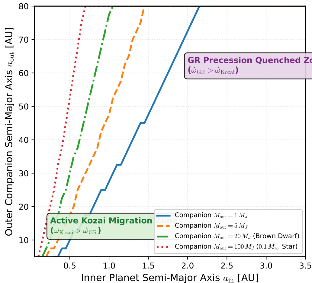
(b) Kozai Migration vs GR Quenching Boundaries
