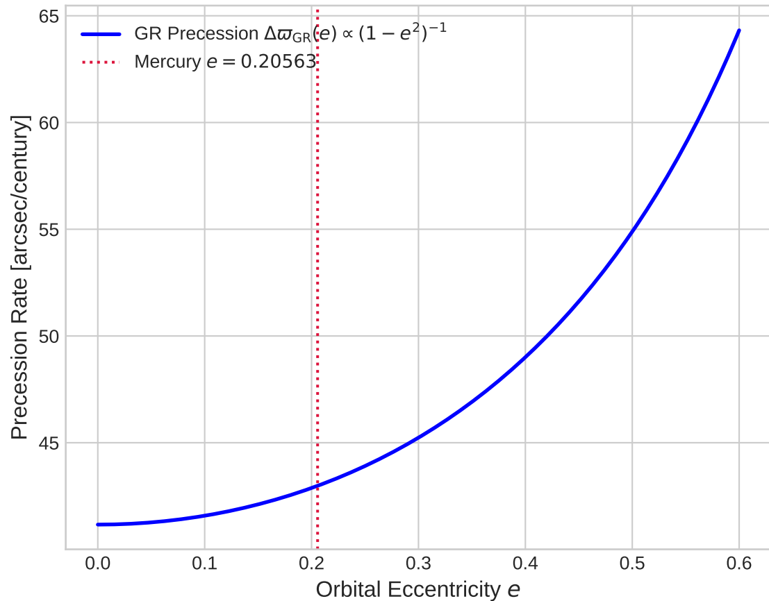
Model Sensitivity: Precession vs Eccentricity
