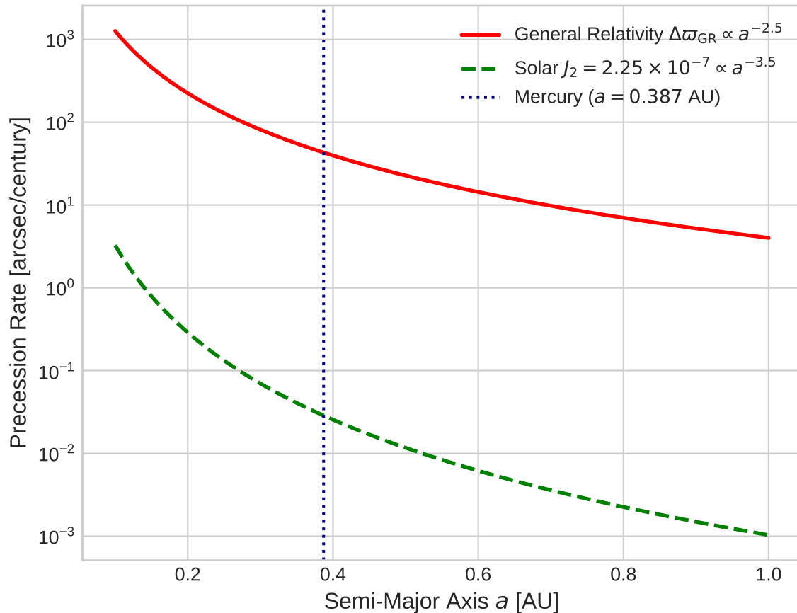
Model Sensitivity: Precession vs Distance
