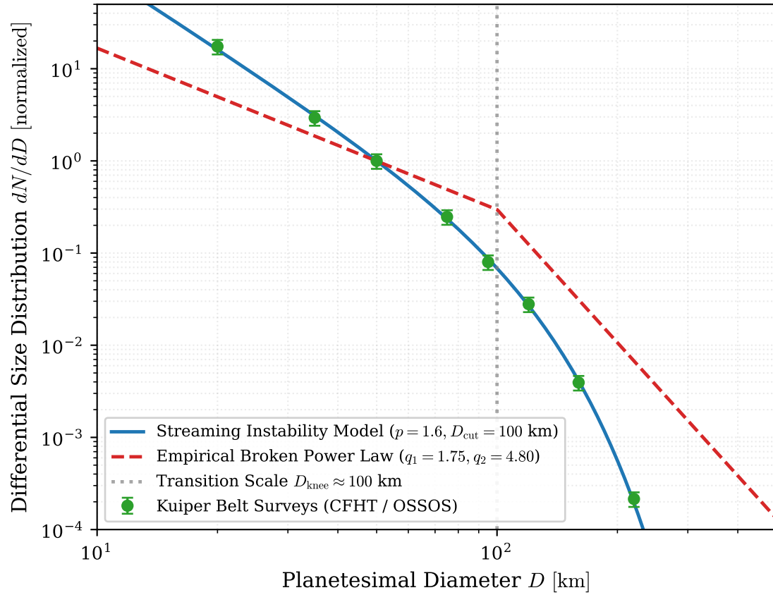
\textbf{(a) Planetesimal Size Distribution dN/dD }
