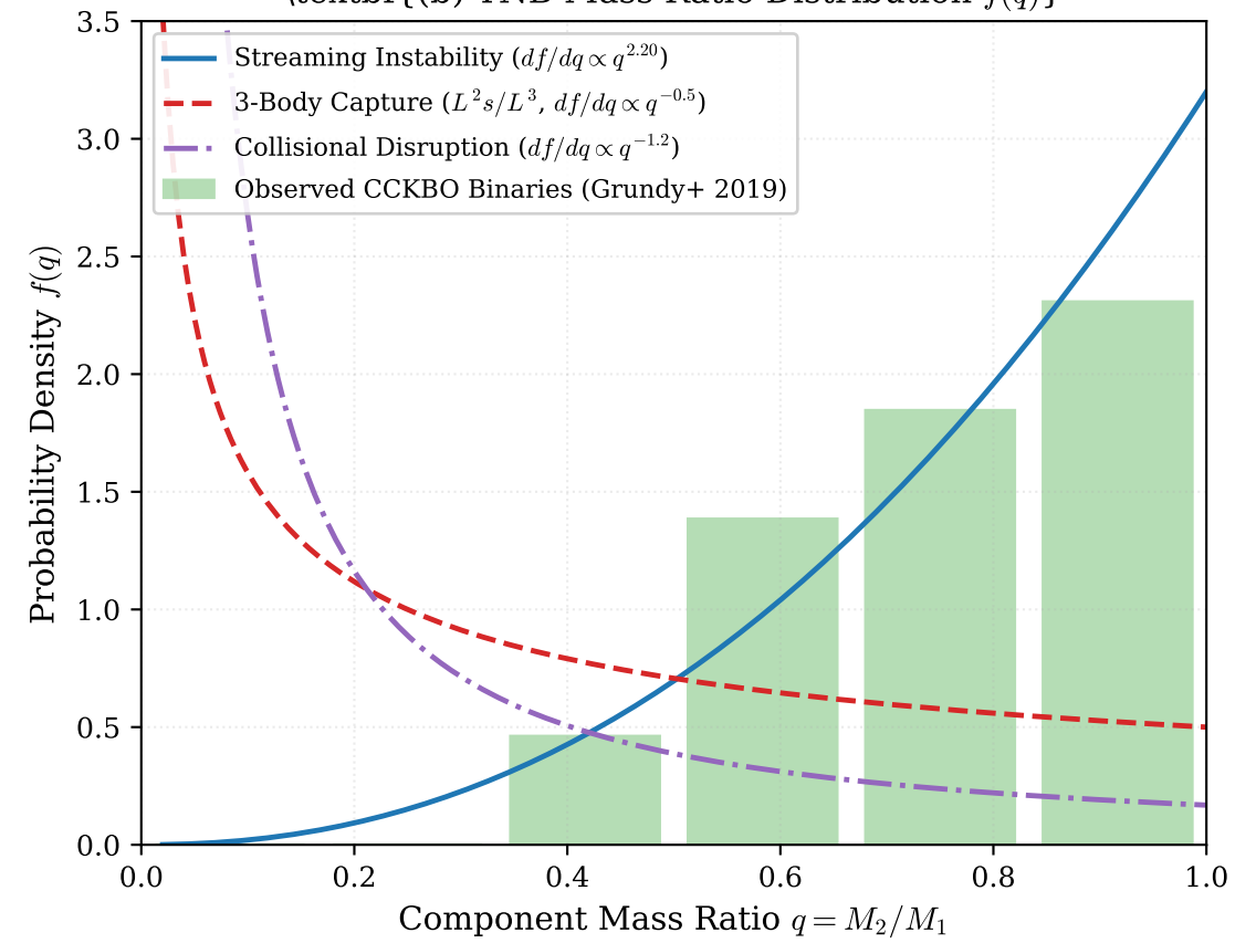
\textbf{(b) TNB Mass Ratio Distribution f(q) }
