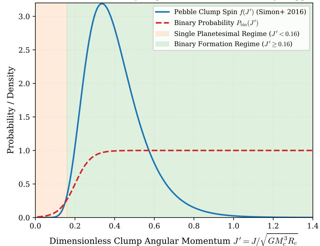
\textbf{(b) Pebble Clump Angular Momentum \& Binary Trigger}
