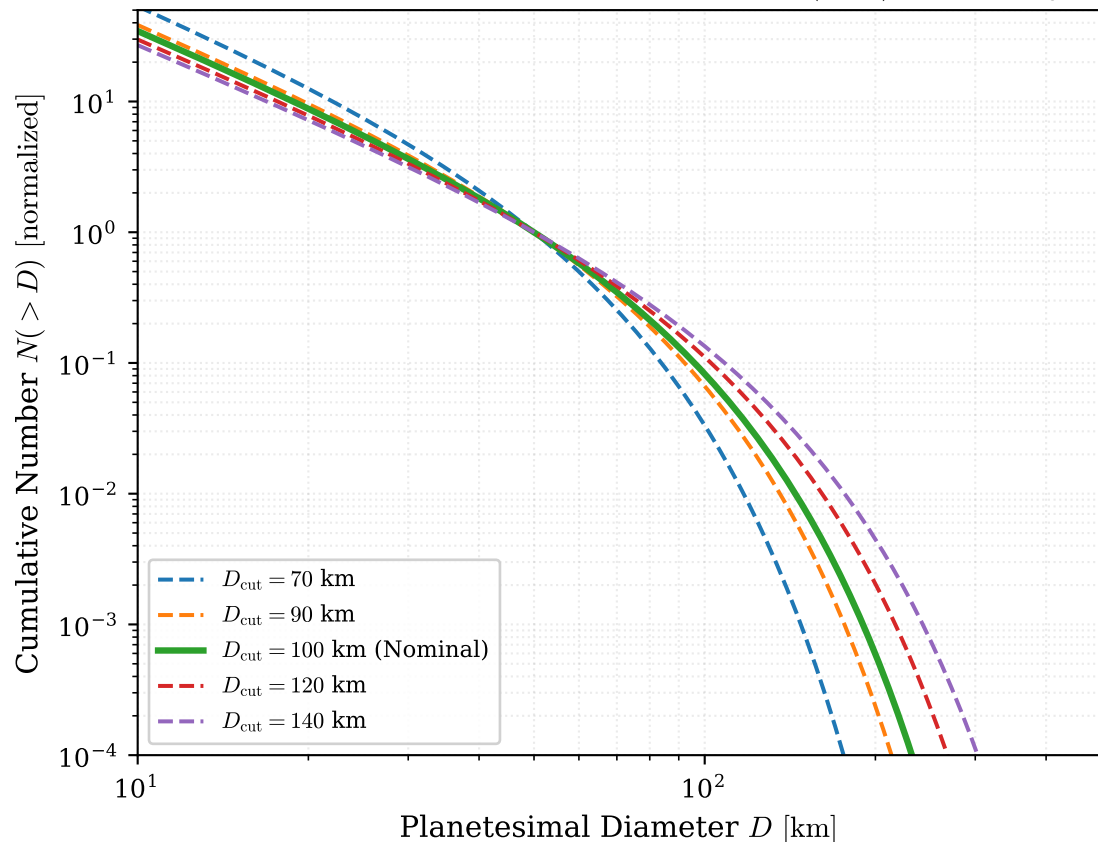
\textbf{(a) Cumulative Size Distribution N(>D) Sensitivity}
