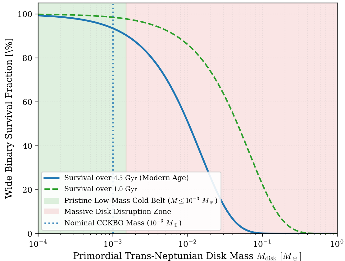
\textbf{(d) 4.5 Gyr Binary Preservation \& Low Disk Mass}
