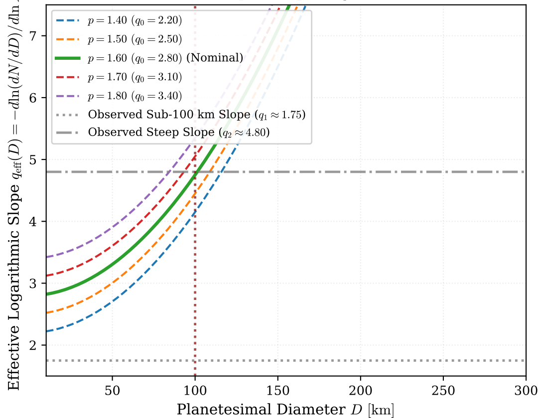
\textbf{(c) Smooth Slope Steepening Across Knee Scale}
