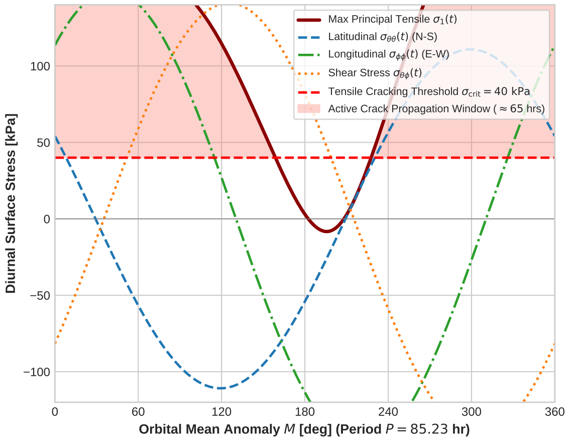
(b) Diurnal Stress Tensor Cycle at ( -45^\circ N, 200^\circ E)
