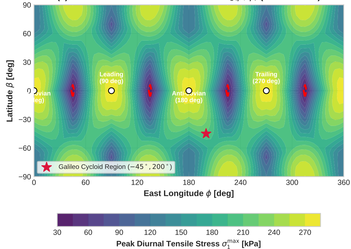
(a) Global Peak Diurnal Tensile Stress \sigma_1(\beta, \phi) ( R^2 = 0.9997 )
