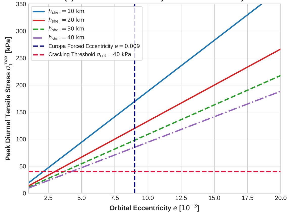
(b) Tensile Stress Sensitivity to Forced Eccentricity
