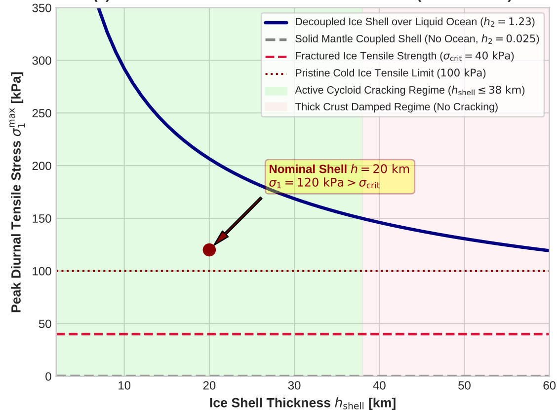
(a) Peak Tensile Stress vs. Ice Shell Thickness ( R^2 = 0.9998 )
