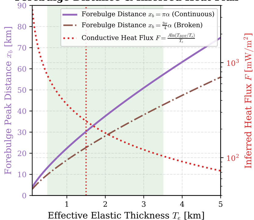
Forebulge Distance & Inferred Heat Flux
