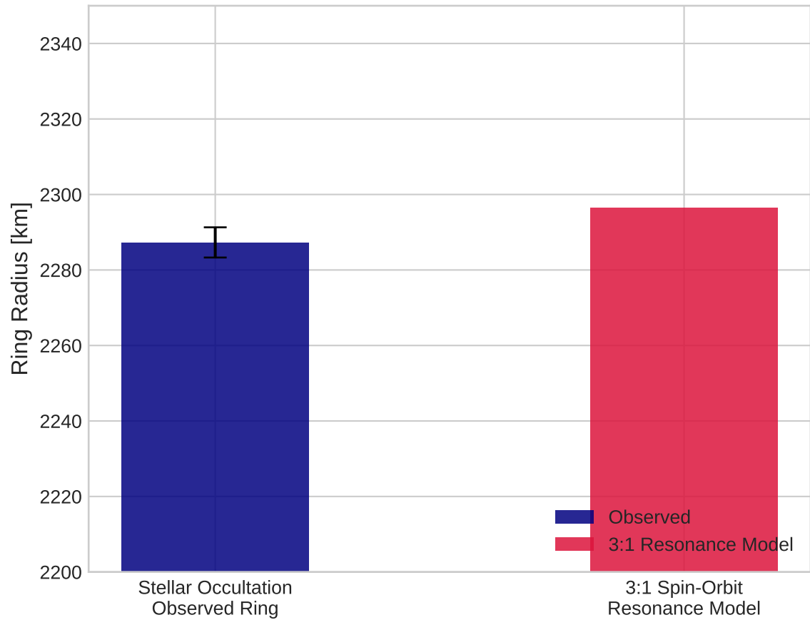
Haumea Ring Radius Model Matching
