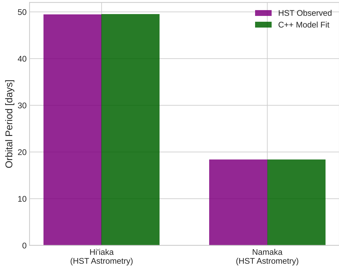
Haumea Satellite Orbital Periods
