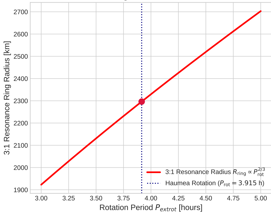
Model Choice: Ring Resonance vs Rotation Period
