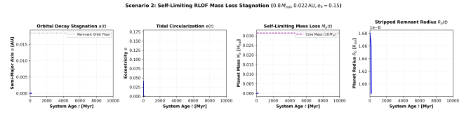
Figure 2: Scenario 2: Self-Limiting RLOF Stagnation ( 0.8 M_{\text{Jup}} , 0.022 \text{ AU} , e_0 = 0.15 ). Coupled time evolution of semi-major axis a(t) , eccentricity e(t) , mass M_p(t) , and radius R_p(t) . Tidal circularization damps eccentricity to zero ( e \rightarrow 0 ), while envelope stripping drives structural contraction ( R_p \propto M_p^{0.6} ), halting mass loss and allowing the planet to survive as a circularized USP remnant.
