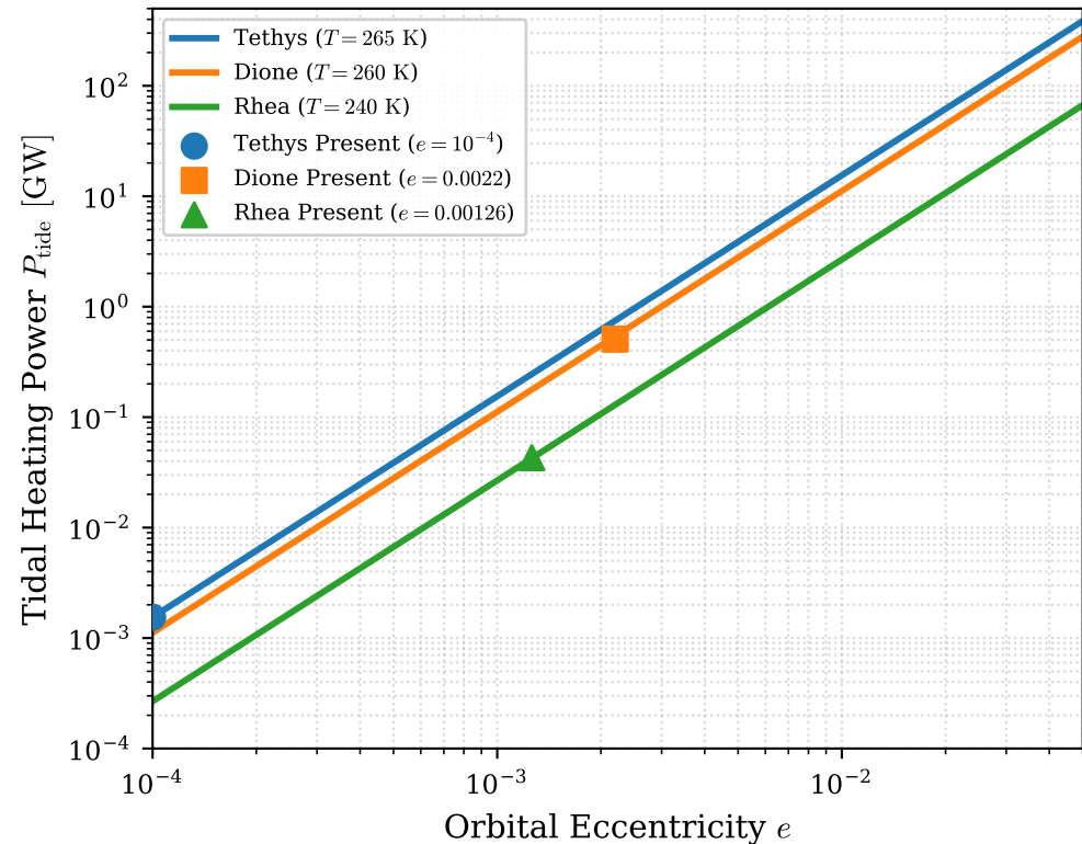
(a) Tidal Power Scaling with Orbital Eccentricity
