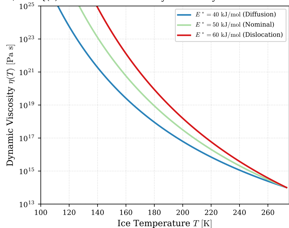
(c) Arrhenius Ice Viscosity Sensitivity to Activation Energy
