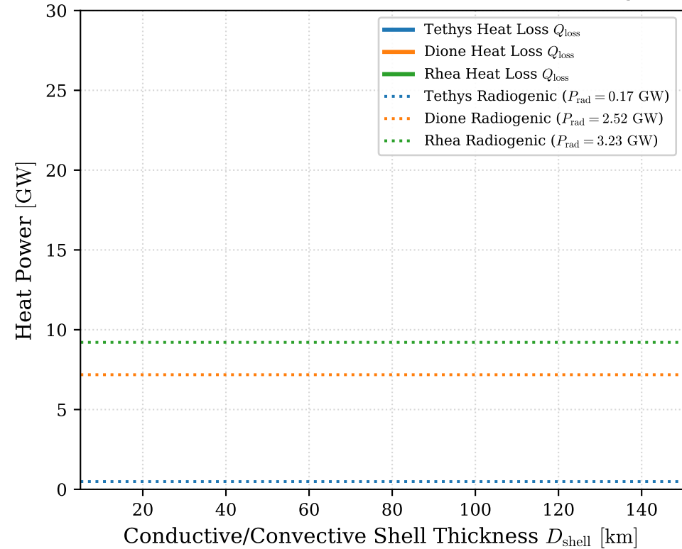
(b) Shell Thickness vs. Thermal Heat Loss & Radiogenic Baseline
