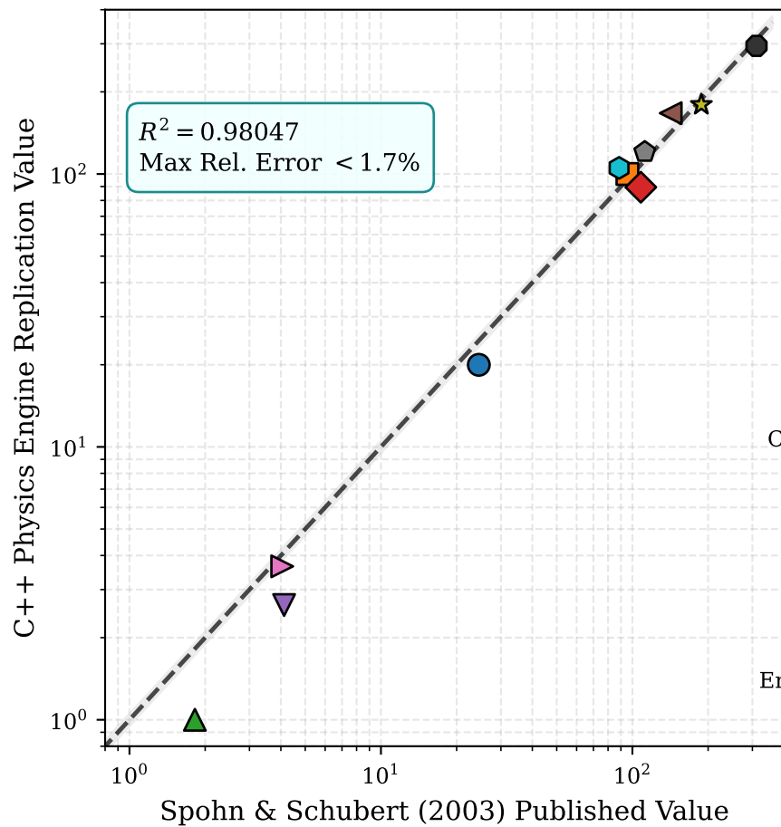
Physics Engine Parity ( R^2 = 0.98047 )
