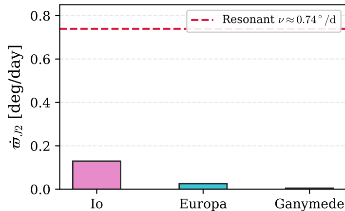
(c) Secular Precession Rates
