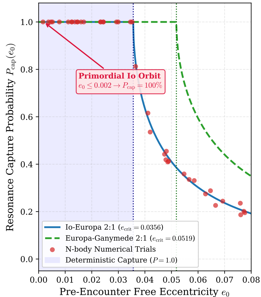
(a) Resonance Capture Probability
