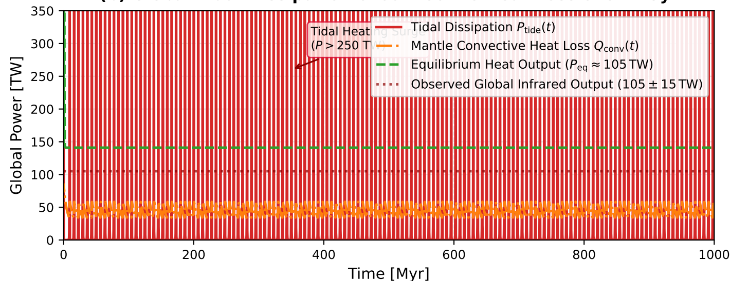
(b) Global Tidal Dissipation & Convective Heat Loss over 1 Gyr
