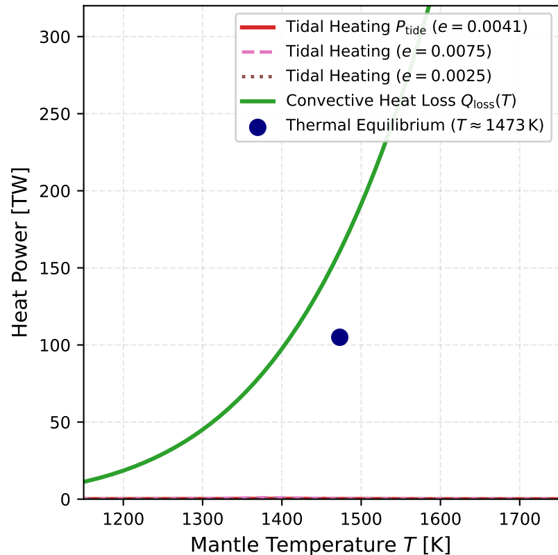
(b) Mantle Thermal Balance & Stability Crossing
