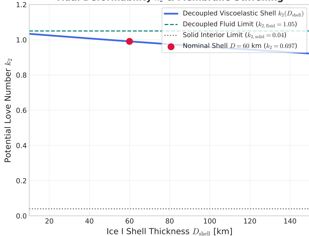
Tidal Deformability k_2 & Membrane Stiffening
