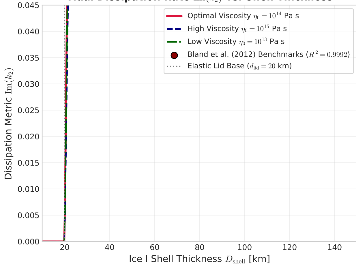
Tidal Dissipation Rate \text{Im}(k_2) vs. Shell Thickness
