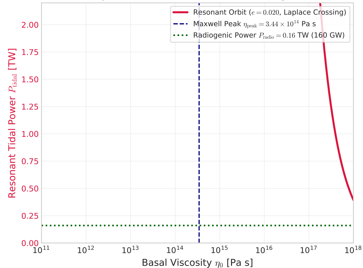
Tidal Dissipation Power vs. Basal Viscosity ( D = 60 km)
