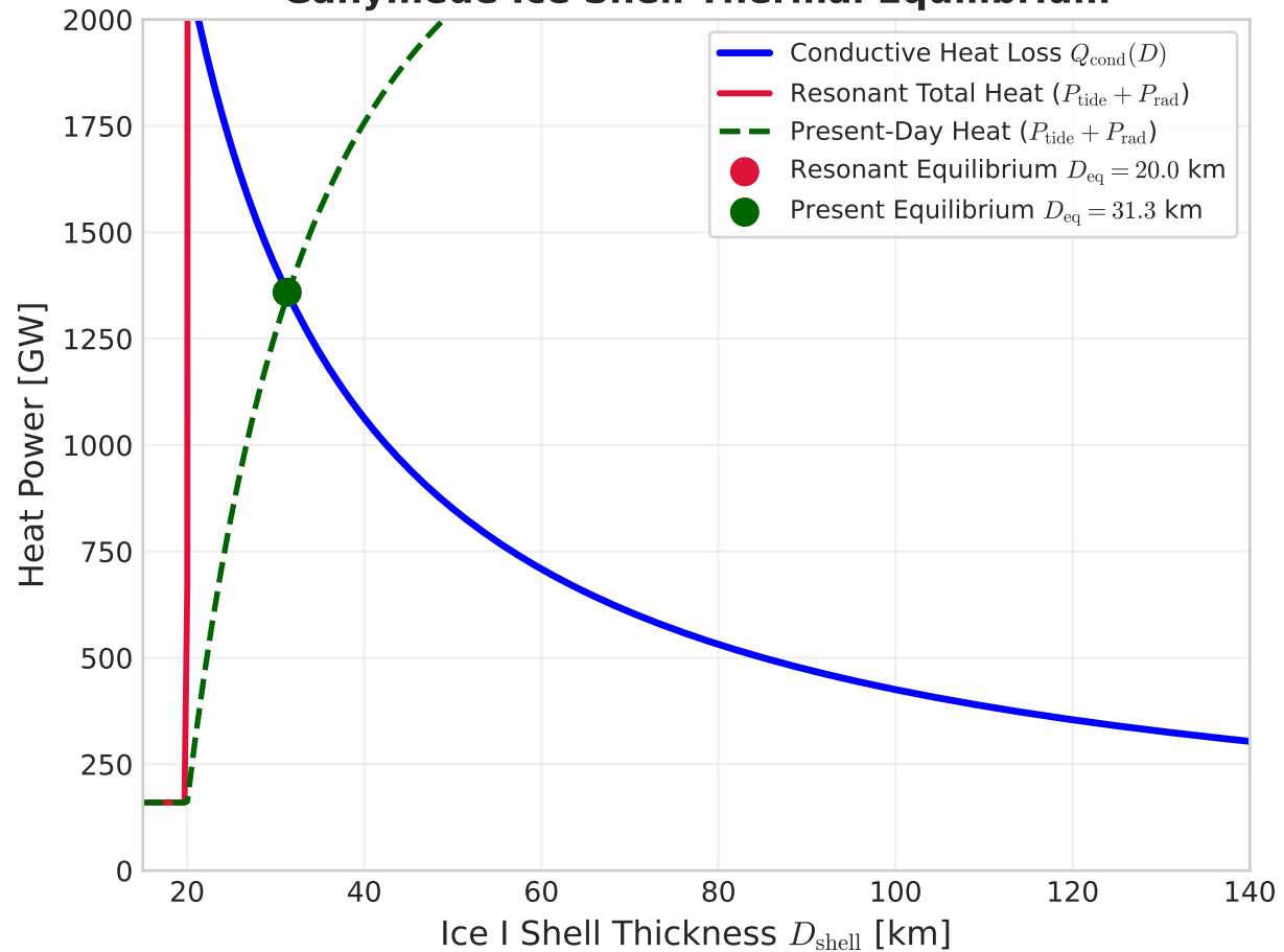
Ganymede Ice Shell Thermal Equilibrium
