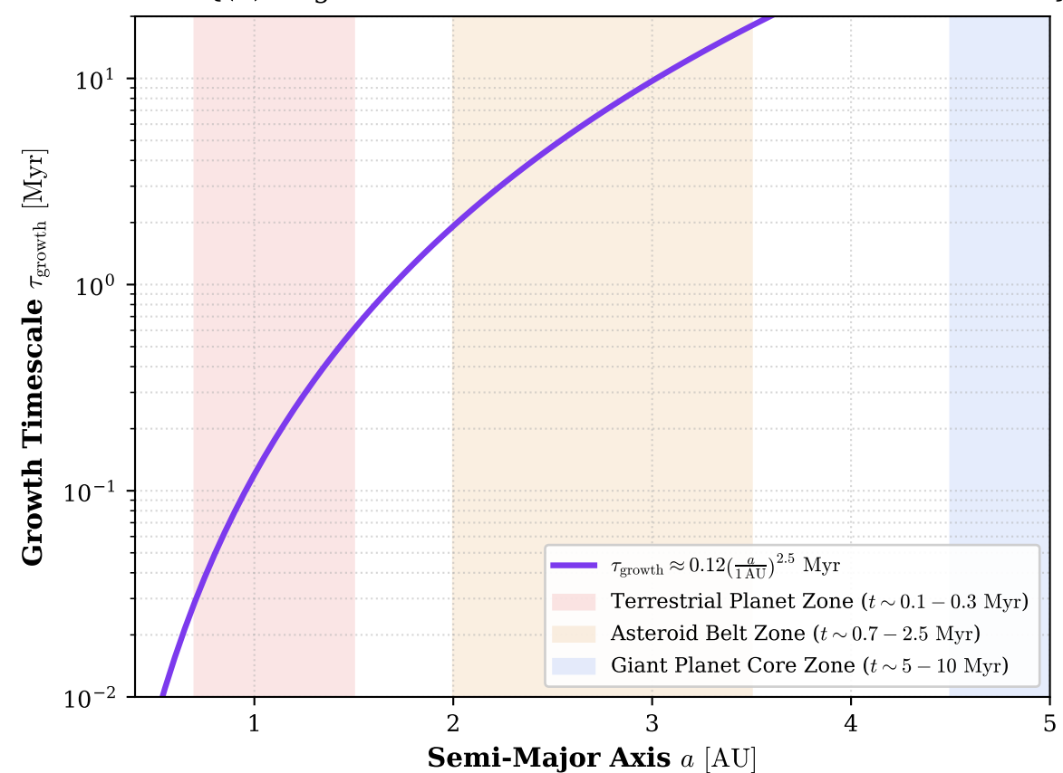
\textbf{(b) Oligarch Formation Timescale vs Heliocentric Distance}
