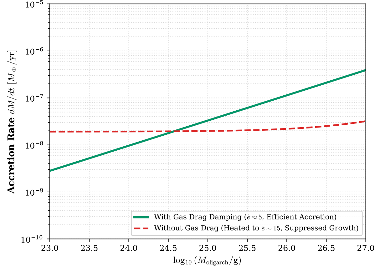
\textbf{(d) Gas Drag Accretion Boost via Gravitational Focusing}
