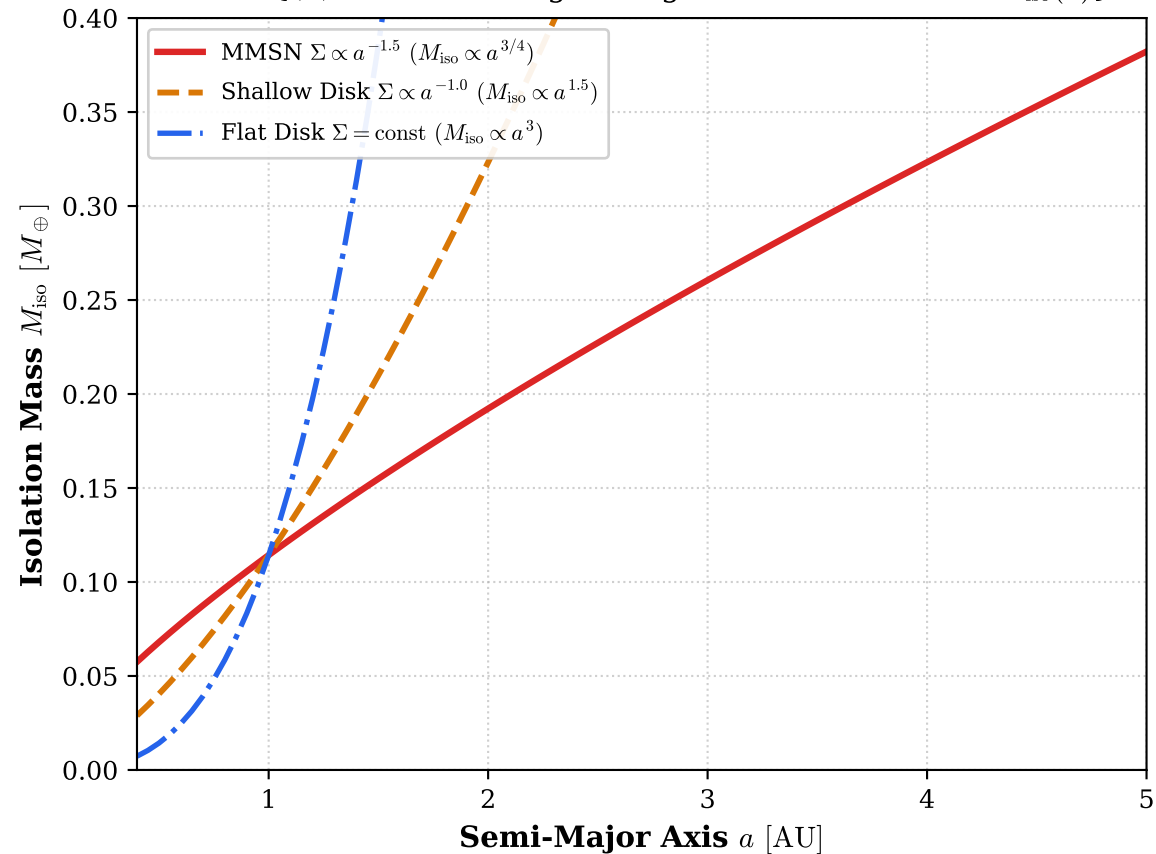
\textbf{(a) Radial Scaling of Oligarch Isolation Mass M_{\text{iso}}(a) }
