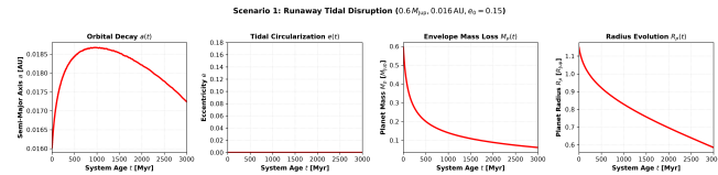
Figure 1: Scenario 1: Runaway Tidal Disruption ( 0.6 M_{\text{Jup}} , 0.016 \text{ AU} , e_0 = 0.15 ). Coupled time evolution of orbital semi-major axis a(t) , orbital eccentricity e(t) , planetary mass M_p(t) , and radius R_p(t) . Rapid planetary tidal dissipation circularizes the orbit ( e \rightarrow 0 in t \lesssim 100 \text{ Myr} ) prior to runaway RLOF mass loss and tidal engulfment into the host star.
