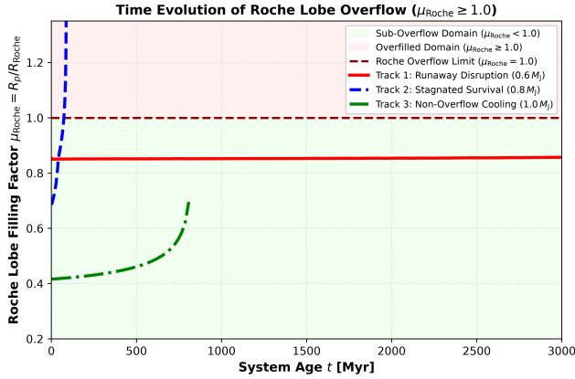
Figure 5: Roche Lobe Radius Contraction and Filling Factor. Time evolution of filling factor \mu_{\text{Roche}}(t) = R_p/R_{\text{Roche}} . Overfilling ( \mu_{\text{Roche}} \geq 1.0 , red shaded region) initiates hydrodynamic mass loss, while sub-overflow ( \mu_{\text{Roche}} < 1.0 , green shaded region) represents stable cooling.
