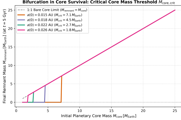
Figure 9: Bifurcation in Core Survival. Final remnant mass M_{\text{remnant}} at t = 5 Gyr as a function of initial core mass M_{\text{core}} across orbital separations a(0) \in [0.015, 0.026] AU. Cores below M_{\text{core,crit}} undergo total hydrodynamic disruption ( M_{\text{remnant}} = 0 ).
