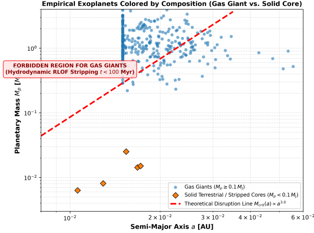
Figure 7: Empirical Gas Giant Truncation Boundary. Observed transiting exoplanet population from hot_jupiter.db overlaid with the theoretical RLOF disruption boundary (red dashed curve), color-coded by planet composition (blue circles: Gas Giants M_p \geq 0.1 M_{\text{Jup}} ; orange diamonds: Solid Terrestrial Cores M_p < 0.1 M_{\text{Jup}} ).
