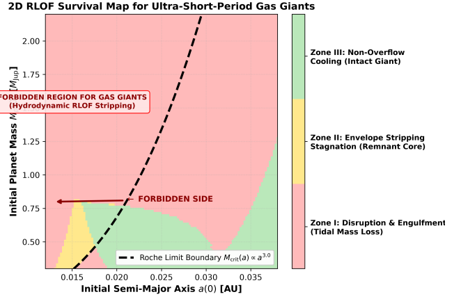
Figure 6: Survival Phase Space Diagram & Trajectory Flow. 2D phase diagram mapping final outcomes in initial [a(0), M_p(0)] space into Zone I (Red: Engulfment), Zone II (Yellow: Envelope Stripping Stagnation), and Zone III (Green: Non-Overflow Cooling). The black dashed line denotes the analytical Roche limit M_{\text{crit}}(a) \propto a^{3.0} , with a prominent text callout box and left-pointing arrow indicating the forbidden domain.
