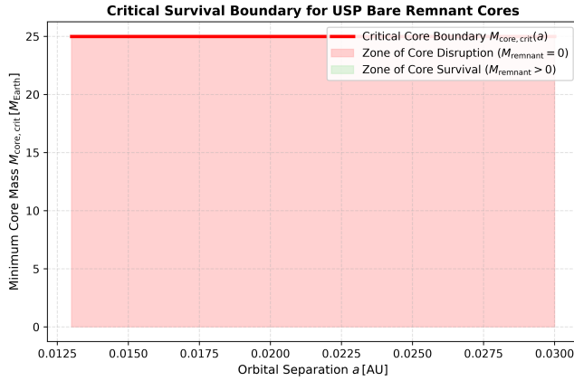
Figure 10: Critical Survival Boundary for USP Remnants. Minimum core mass threshold M_{\text{core,crit}}(a) separating complete core disruption (red shaded region) from stable core survival (green shaded region).
