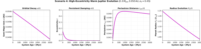
Figure 4: Scenario 4: High-Eccentricity Warm Jupiter Evolution ( 1.0 M_{\text{Jup}}, 0.050 \text{ AU}, e_0 = 0.45 ). Coupled time evolution of semi-major axis a(t) , persistent tidal eccentricity damping e(t) , periastron separation r_{\text{peri}}(t) = a(t)(1 - e(t)) , and radius contraction R_p(t) . For wider orbits ( a_0 = 0.050 \text{ AU} ), tidal circularization timescales \tau_e \propto a^{13/2} exceed \sim 3 \text{ Gyr} , allowing non-zero eccentricity to persist into multi-Gyr system ages.
