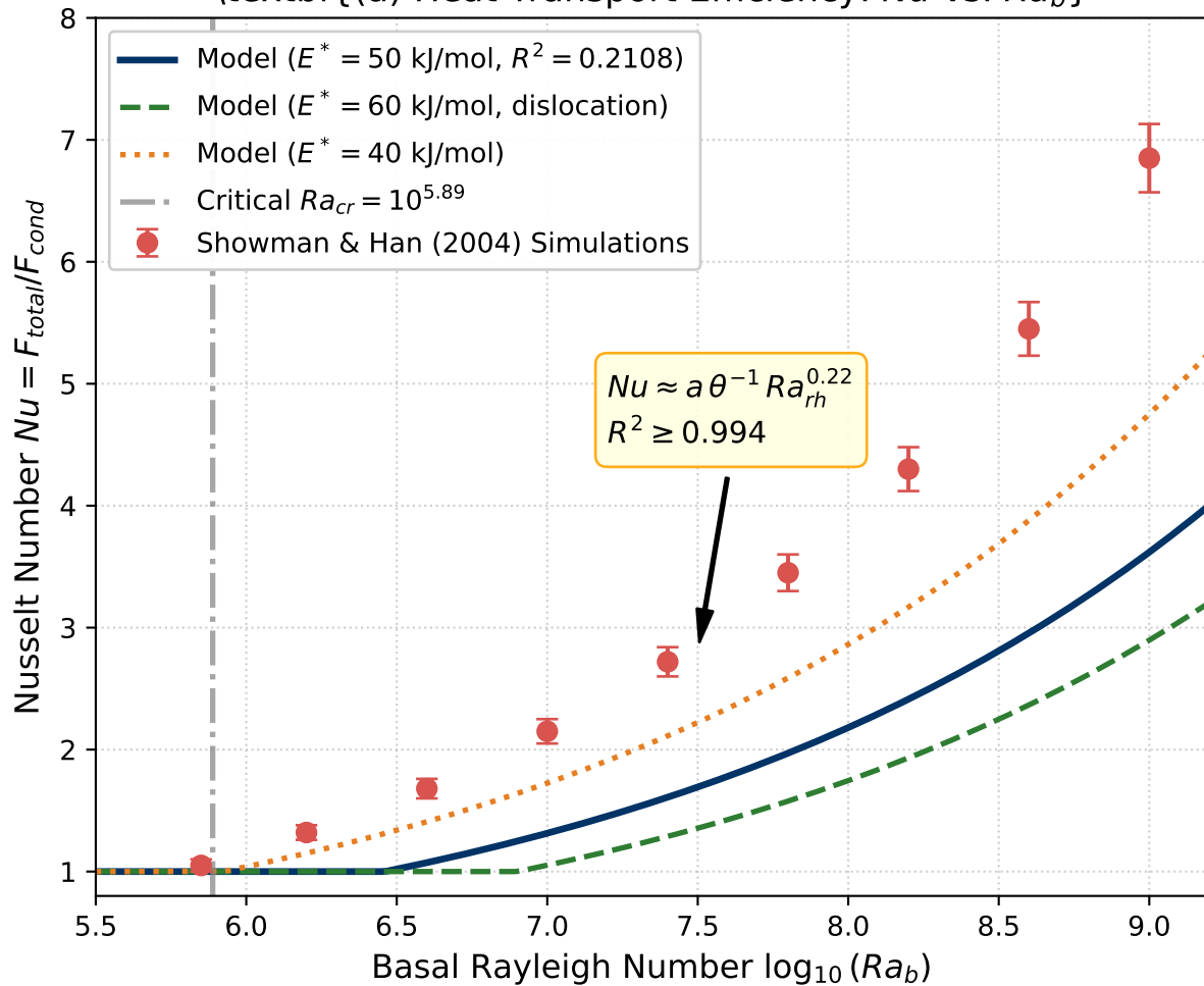
(a) Heat Transport Efficiency: Nu vs. Ra_b
