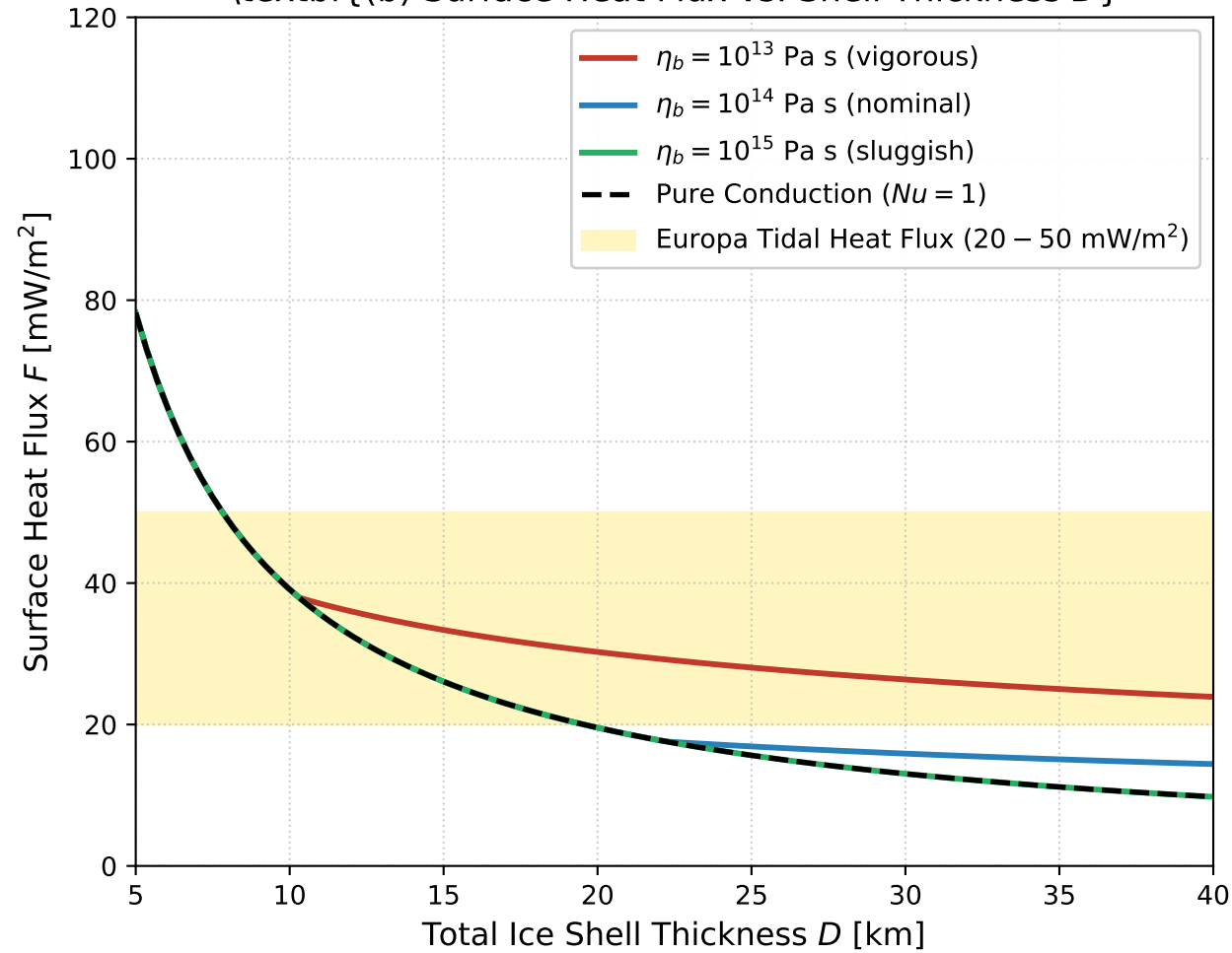
(b) Surface Heat Flux vs. Shell Thickness D
