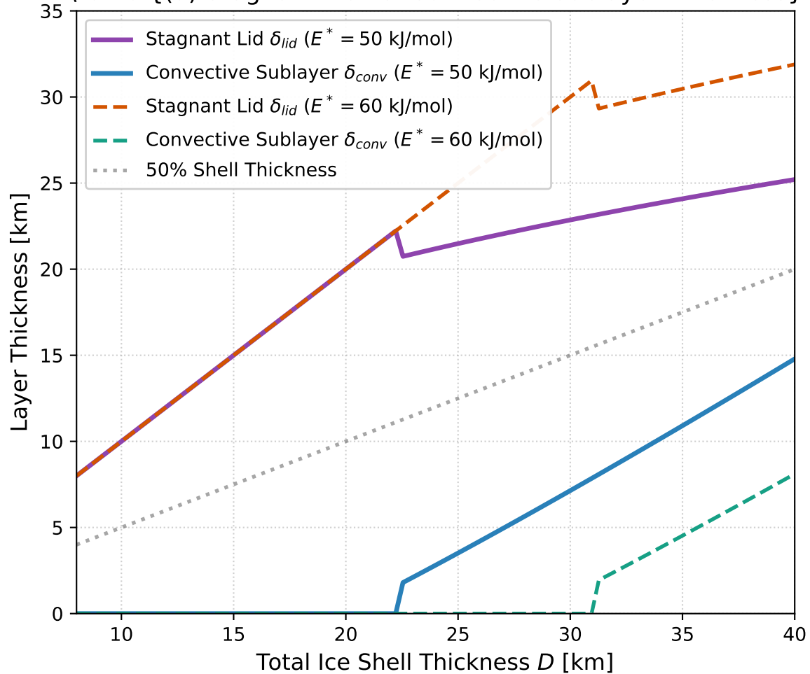
(a) Stagnant Lid vs. Convective Sublayer Thickness
