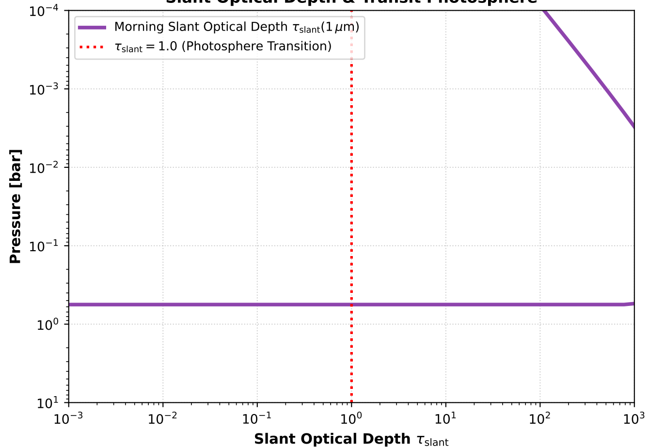
Slant Optical Depth & Transit Photosphere
