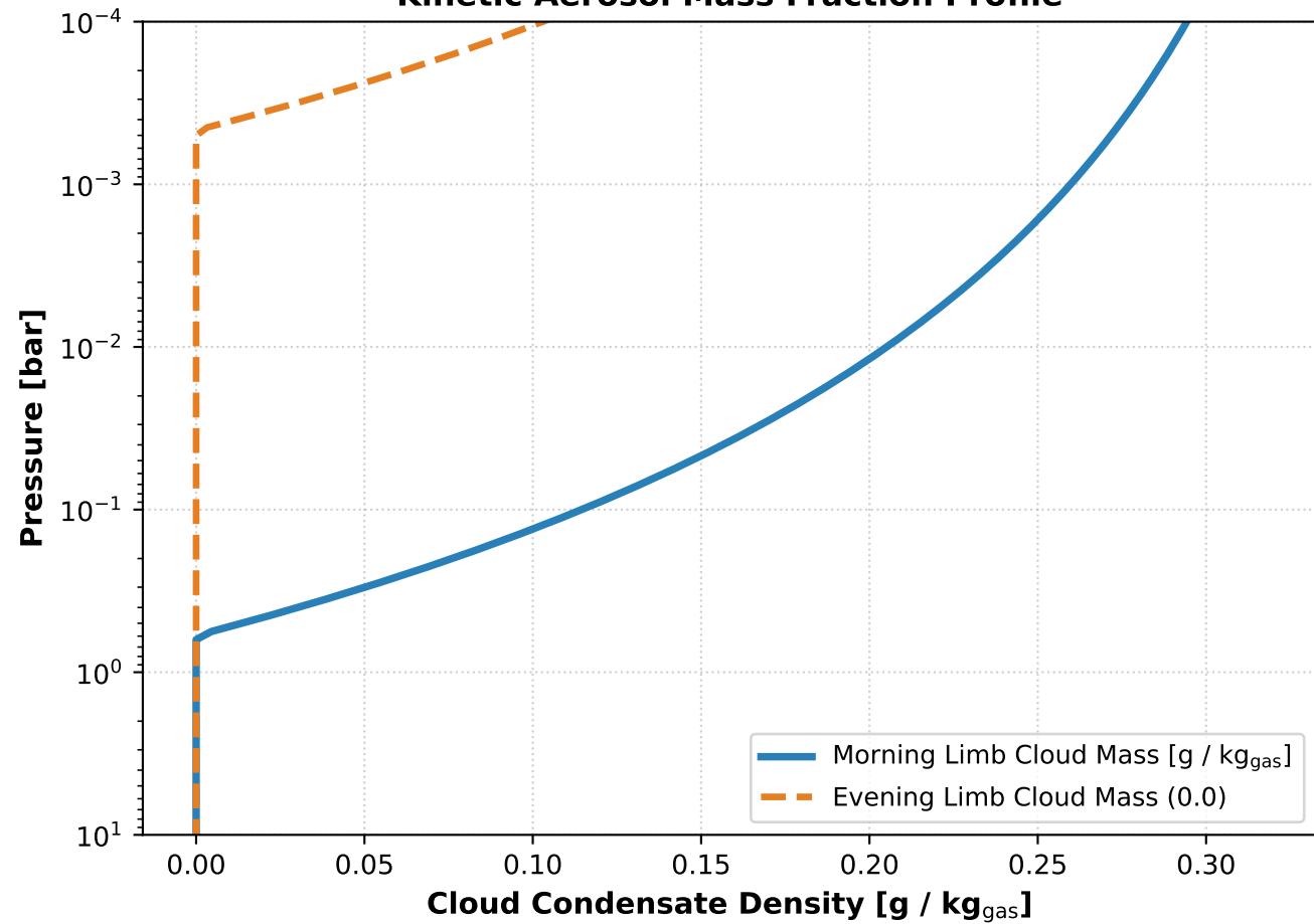
Kinetic Aerosol Mass Fraction Profile
