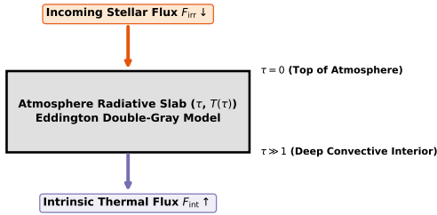
Figure 17: Two-stream double-gray radiative boundary geometry under stellar irradiation.
