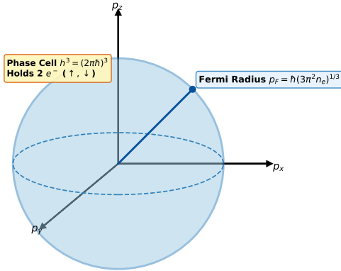
Derivation A3: 3D Quantum Phase Space Fermi Sphere
