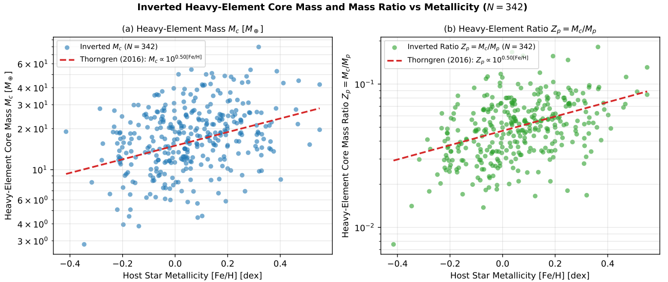
Figure 13: Dual-panel core mass inversion analysis across all N = 342 confirmed transiting Hot Jupiters: (a) Absolute heavy-element core mass M_c [ M_{\oplus} ] vs host star metallicity [\text{Fe}/\text{H}] [dex], and (b) Dimensionless heavy-element core mass fraction Z_p = M_c/M_p vs [\text{Fe}/\text{H}] [dex], compared against the empirical Thorngren et al. (2016) power-law trend.
