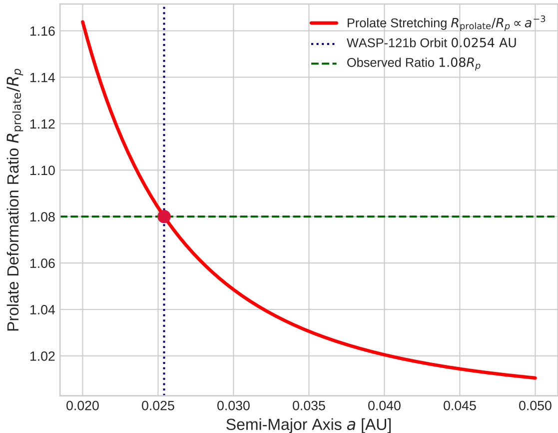
Model Choice: Tidal Distortion vs Semi-Major Axis
