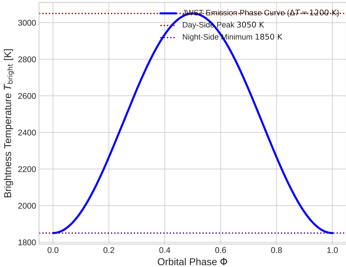
Model Choice: Thermal Phase Curve Emission
