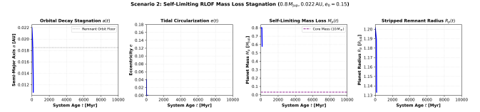
Figure 2: Scenario 2: Self-Limiting RLOF Stagnation ( 0.8 M_{\text{Jup}}, 0.022 \text{ AU}, e_0 = 0.15 ). Coupled time evolution of semi-major axis a(t) , eccentricity e(t) , mass M_p(t) , and radius R_p(t) . Tidal circularization damps eccentricity to zero ( e \rightarrow 0 ), while envelope stripping drives structural contraction ( R_p \propto M_p^{0.6} ), halting mass loss and allowing the planet to survive as a circularized USP remnant.
