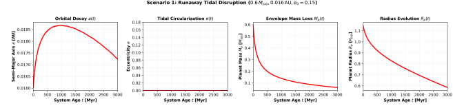
Figure 1: Scenario 1: Runaway Tidal Disruption ( 0.6 M_{\text{Jup}}, 0.016 \text{ AU}, e_0 = 0.15 ). Coupled time evolution of orbital semi-major axis a(t) , orbital eccentricity e(t) , planetary mass M_p(t) , and radius R_p(t) . Rapid planetary tidal dissipation circularizes the orbit ( e \rightarrow 0 in t \lesssim 100 \text{ Myr} ) prior to runaway RLOF mass loss and tidal engulfment into the host star.
