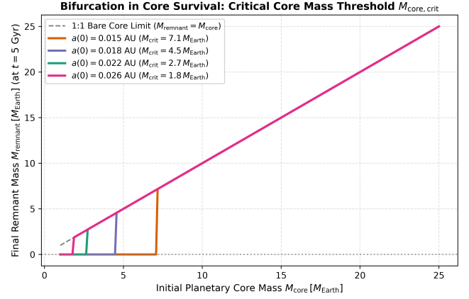
Figure 9: Bifurcation in Core Survival. Final remnant mass M_{\text{remnant}} at t = 5 Gyr as a function of initial core mass M_{\text{core}} across orbital separations a(0) \in [0.015, 0.026] AU. Cores below M_{\text{core, crit}} undergo total hydrodynamic disruption ( M_{\text{remnant}} = 0 ).
