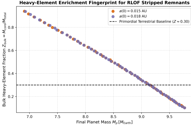
Figure 11: Heavy-Element Enrichment Fingerprint. Final bulk heavy-element fraction Z_{\text{bulk}} \equiv M_{\text{core}}/M_{\text{total}} of surviving USP remnants, compared against the baseline of primordially accreted terrestrial planets ( Z \approx 0.30 ).
