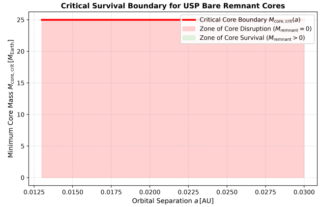
Figure 10: Critical Survival Boundary for USP Remnants. Minimum core mass threshold M_{\text{core, crit}}(a) separating complete core disruption (red shaded region) from stable core survival (green shaded region).
