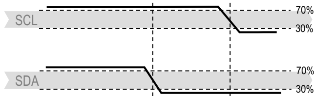
Figure18 Start Transmit State (S) - When SCL is at high level, SDA is converted from high level to low level. The start state is a special bus state controlled by the main engine, indicating the start of slave machine transit (after Start, BUS is generally considered to be in a busy state).
