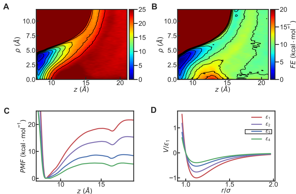
Figure S5: FES of original (A) and fast unbinding model, \epsilon_3 (B), as function of \rho and z . (C) Projection of FES onto transverse distance, z , for all models. (D) LJ potential for interactions between cavity and ligand atoms (CP-CF) in original and modified models, potential was scaled by \epsilon_1 (see Table 3) and distance was scaled by \sigma .
