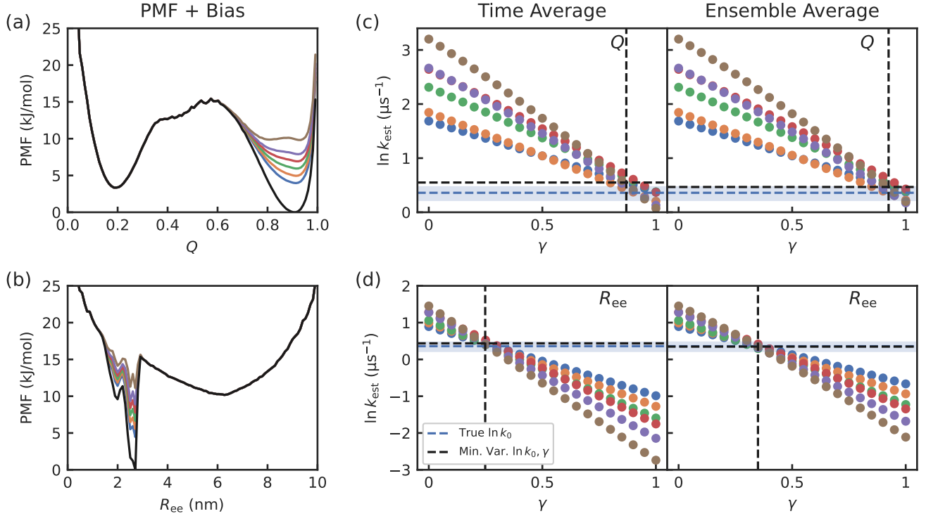
Figure S3: (a), (b) The PMFs of the protein G model for Q and R_{ee} . The unbiased PMF is shown in black while the biased PMF for each bias level is colored. (c), (d) The values of \ln k_0 predicted by Eq. 8 for each set of simulations for various values of \gamma , by approximating the expected value \langle e^{\beta\gamma V} \rangle using the time average of the simulation average (left) and the directly estimated ensemble average (right).
