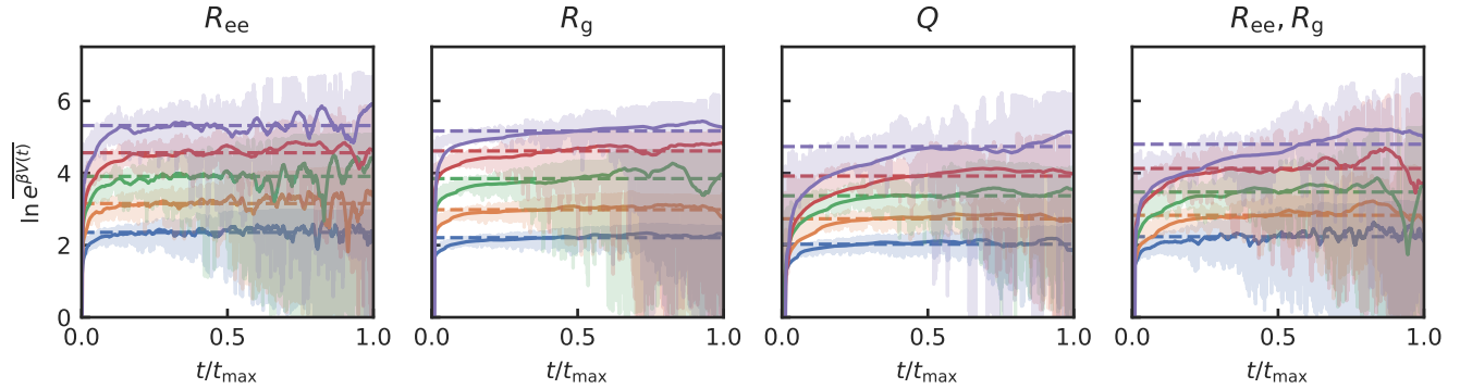
Figure S1: The log of the value of e^{\beta V(t)} averaged over all simulations in each set (low opacity). The solid lines represent the log of the time average of e^{\beta V(t)} over a window of 25000 steps, and the horizontal dashed lines represent the time average from 0 up to the maximum transition time, which approximates the log of the ensemble average \ln \langle e^{\beta V} \rangle in the folded state.
