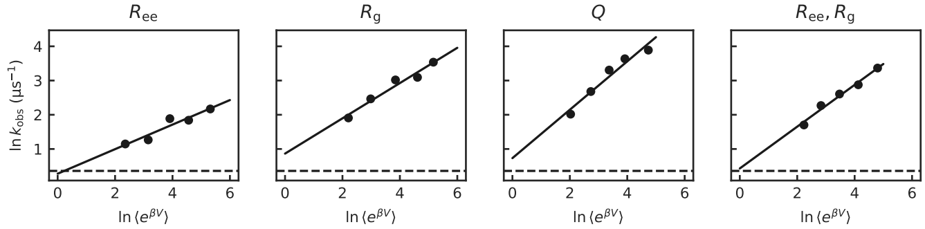
Figure S2: The logarithm of the observed rate plotted against \ln \langle e^{\beta V} \rangle in the folded state of the protein G model, estimated as the log of the time average of e^{\beta V(t)} . The horizontal dashed line represents the value of \ln k_0 . Increasing \ln \langle e^{\beta V} \rangle for poor CVs has less of an effect on \ln k_{obs} than for good CVs. The EATR-slope approach takes the y-intercept of the best fit line to be the estimate for \ln k_0 and the slope to be the estimate for \gamma .
