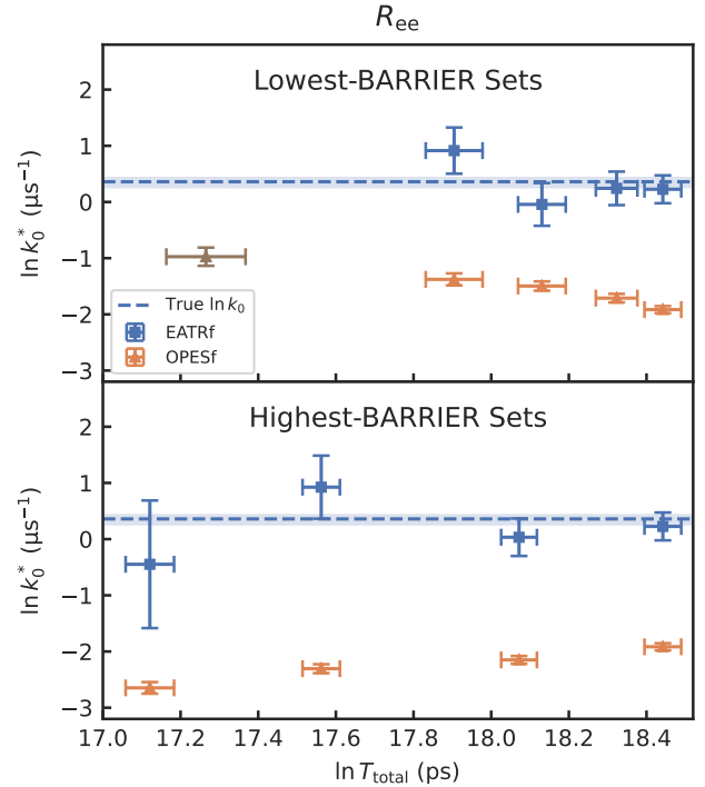
Figure 5: The predicted value of \ln k_0 from EATR-flooding and OPES-flooding on the R_{\text{ee}} CV with the lowest (top) and highest (bottom) values for \Delta E with 100 simulations per set. The blue dashed line represents the rate obtained from unbiased simulations. Error bars indicate the standard error in bootstrap analysis.
