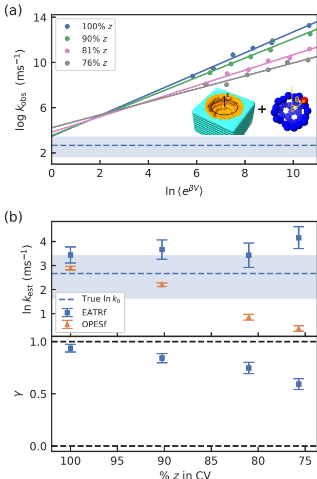
Figure 7: (a) The observed value of the log rate in the simulation sets while biasing a CV defined as linear combinations of z and \theta , plotted against \ln \langle e^{\beta V} \rangle , which acts as a measure of the amount of bias added. For worse CVs that have a larger contribution from \theta , adding the same amount of bias has less of an effect on the observed rate. Solid lines are linear fits to the data, with slopes from top to bottom of 0.94, 0.84, 0.75, and 0.59. (b) The predicted value of \ln k_0 (top) and \gamma (bottom) from EATR-flooding and OPESf while biasing each of the CVs. The x-axis is the value of a^2 where a is the coefficient of z in the linear combination. Mean \gamma values are 0.92, 0.86, 0.68, and 0.57, quite similar to the values of slope in (a), in accordance with the hypothesis in Ref. 24.
