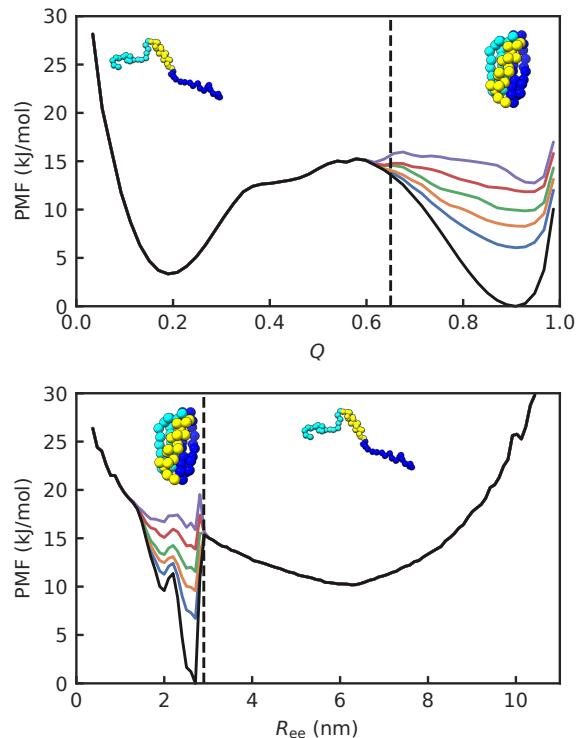
Figure 2: The potential of mean force (PMF) along the fraction of native contacts CV Q (top) and the end-to-end distance CV R_{\text{ee}} (bottom). The colored lines indicate the PMF with the average final biasing potential from OPES with various values of the \Delta E parameter. From bottom to top, \Delta E = 5, 7, 9, 11 , and 13 kJ/mol. The vertical dashed lines represent the boundary of the excluded region.
