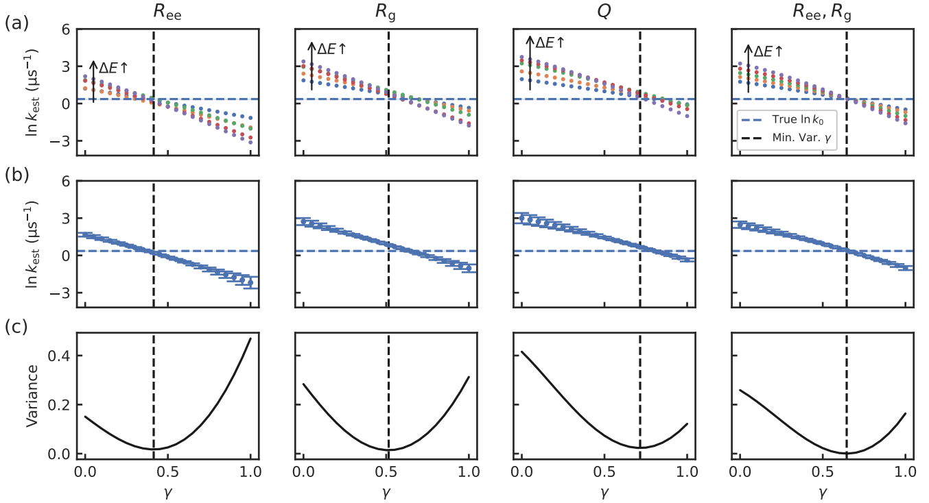
Figure 3: The results of EATR-flooding on the protein G model. (a) The values of \ln k_0 predicted by Eq. 8 for each set of OPES simulations with each \Delta E parameter for various values of \gamma . (b) The value of \ln k_0 averaged over the sets of simulations for each potential value of \gamma . The variance of \ln k_0 across the sets is represented by error bars. (c) The variance in the predicted value of \ln k_0 across the sets of simulations. The horizontal dashed lines represent the true value of \ln k_0 , the uncertainty in which is too small to represent in this plot. The vertical dashed lines represent the minimum variance value of \gamma , which is the value which causes all sets to give the same value of \ln k_0 .
