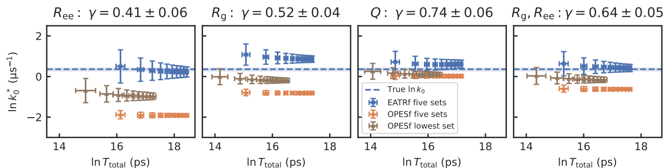
Figure 4: The predicted value of \ln k_0 from EATR-flooding (in blue) and OPES-flooding (in orange) as a function of the logarithm of the total simulation time with the lowest five values for \Delta E . Various numbers of simulations per set, from 5 (left side of each plot) to 100 (right side of each plot). The blue dashed line represents the rate obtained from unbiased simulations. Error bars indicate the standard error in bootstrap analysis.
