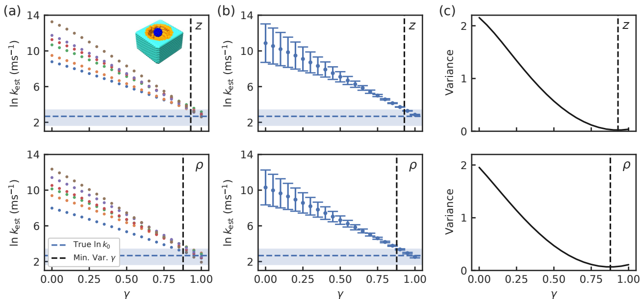
Figure 6: The results of EATR-flooding on the weakened cavity-ligand model. (a) The values of \ln k_0 predicted by Eq. 8 for each set of OPES simulations with each \Delta E for various values of \gamma . (b) The value of \ln k_0 averaged over the sets for each value of \gamma . The variance of \ln k_0 across the sets is represented by error bars. (c) The variance in the predicted value of \ln k_0 across the sets of simulations. The horizontal dashed lines represent the true value of \ln k_0 with the 95% credible interval. The vertical dashed lines represent the minimum variance value of \gamma .
