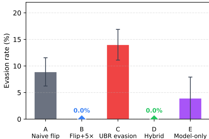
(a) Attack-phase evasion
