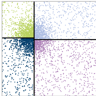
domain decomp., rebalanced
